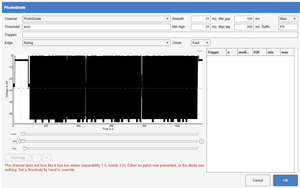
Figure 7.3: Photodiode on a RIFT recording. The diode here follows a 60 Hz flicker rather than a patch that turns on and off, and after smoothing the signal has no two distinct states, so the step reports that, instead of reporting onsets.
