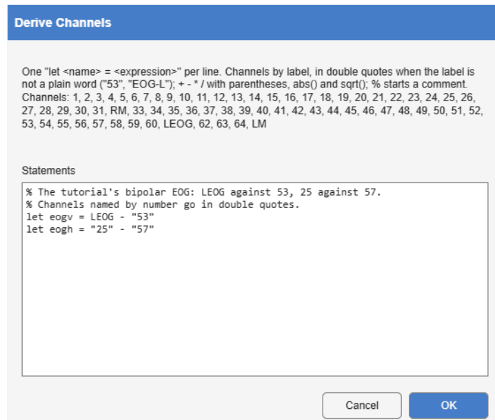
Figure 20.1: The Derive Channels step of the template: the bipolar EOG channels, with the numbered channels in double quotes.
