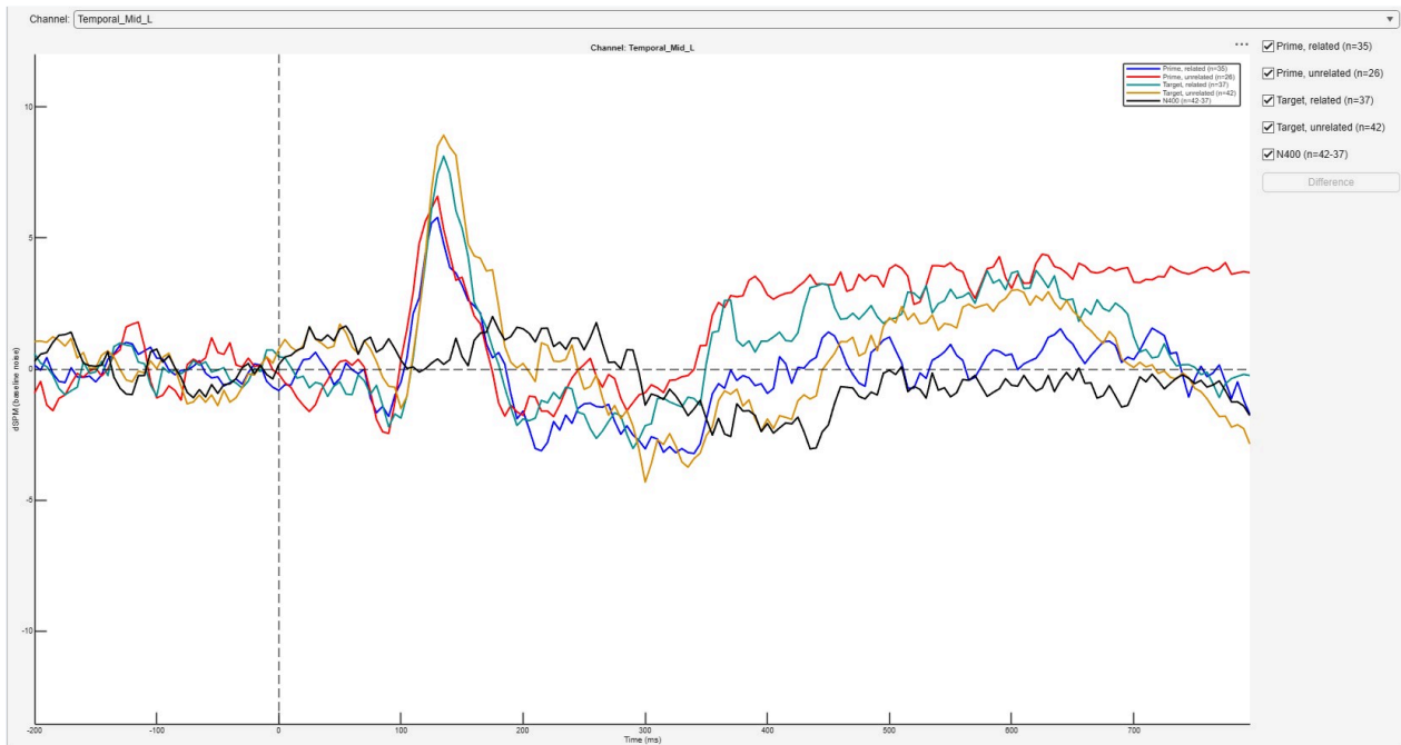
Figure 10.17: The N400 bins in the left middle temporal gyrus (AAL's Temporal_Mid_L), as a signed dSPM time course.
