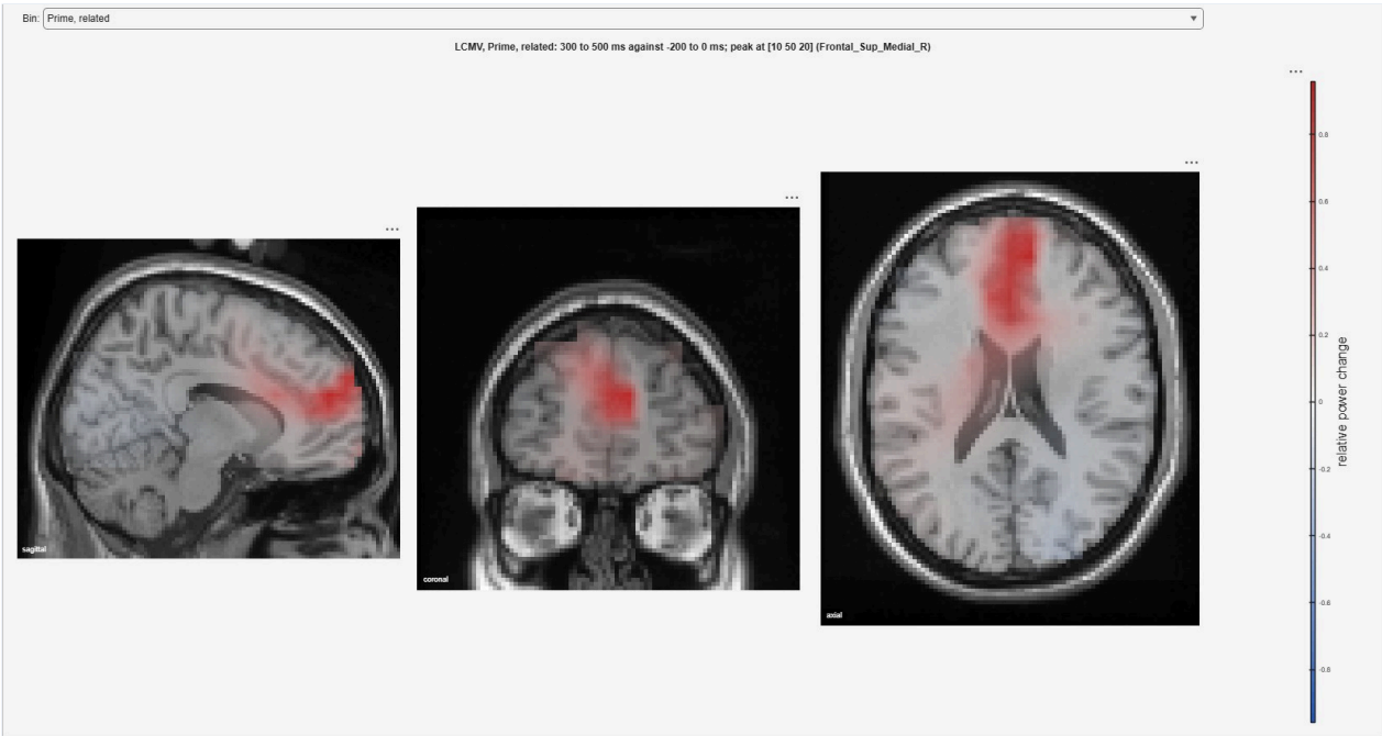
Figure 10.22: The same on a 10 mm volume grid, on slices of the template MRI through the peak.
