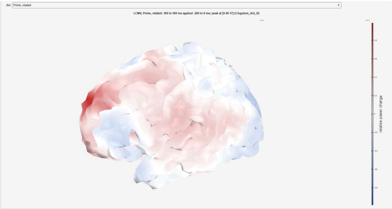
Figure 10.21: LCMV power change from -200 to 0 ms to 300 to 500 ms in the N400 data, on the cortical sheet.
