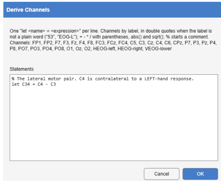
Figure 7.12: Derive Channels on the ERP CORE LRP epochs, adding c34 = c4 - c3 , the lateral motor pair; C4 is contralateral to a left-hand response.
