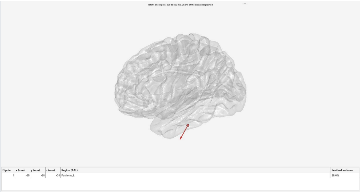
Figure 10.19: A single dipole fitted to the N400 difference from 300 to 500 ms. The residual variance in the title says how much a single dipole leaves unexplained: much, as expected of a component with distributed generators.
