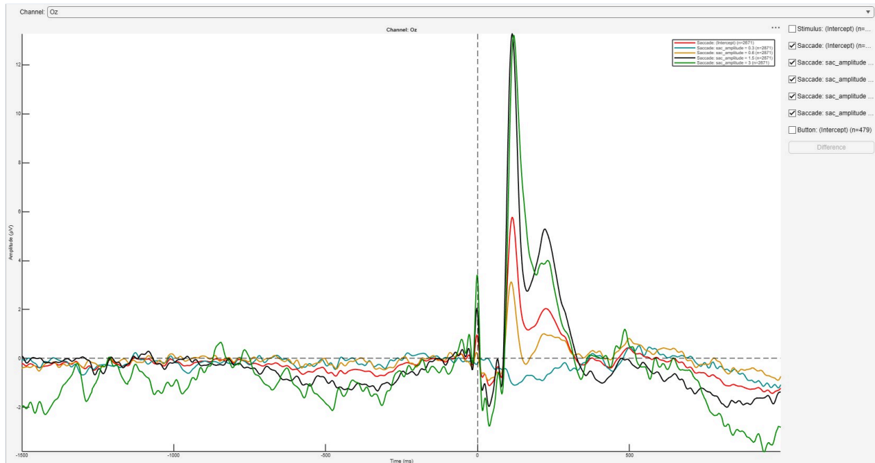
Figure 17.6: The saccade response at Oz for saccades of 0.3, 0.6, 1.5 and 3 degrees, and the intercept (red): the response averaged over this participant's saccades, from the model's terms.
