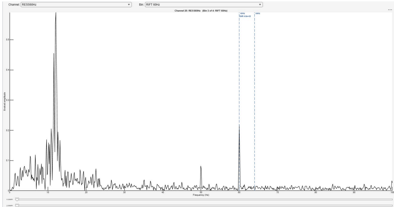
Figure 10.9: The spectrum of the 60 Hz RESS component in the same trials: SNR at 60 Hz about 460, against about 100 at Oz (Figure 10.7), with the 50 Hz line noise largely gone.
