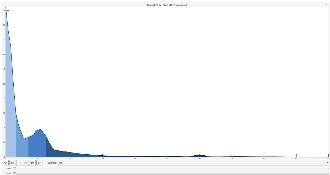
Figure 10.3: The PSD of the N400 epochs at Oz, averaged per bin, with the frequency bands of Section 5.5 shaded beneath it and the alpha peak near 10 Hz.
