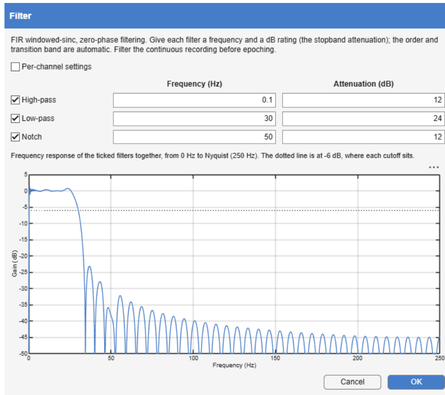
Figure 7.7: Filter , here a combination with a.o., 0.1 Hz high-pass at 12 dB.
