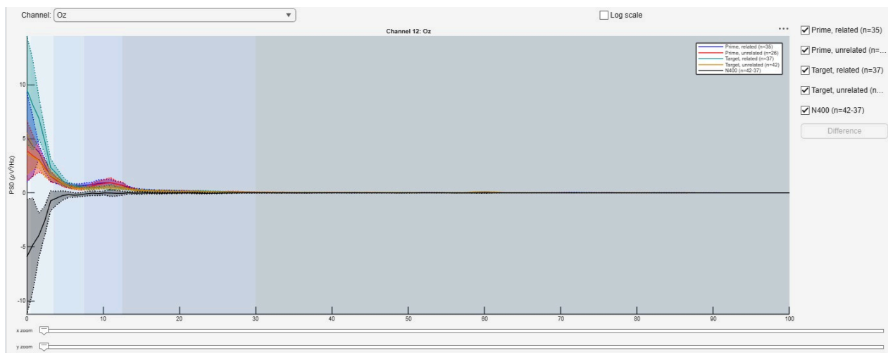
Figure 10.3: The PSD of the N400 epochs at Oz, averaged per bin, with the frequency bands of Section 5.5 shaded beneath it and the alpha peak near 10 Hz.
