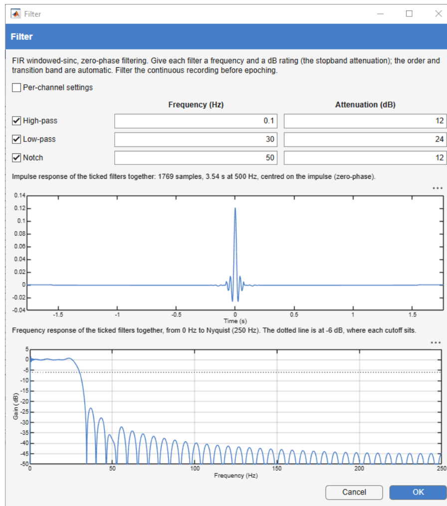
Figure 7.7: Filter, here a combination with a.o., 0.1 Hz high-pass at 12 dB.
