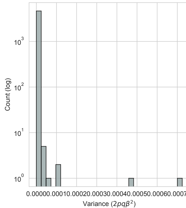
Variance Contribution Dist.
