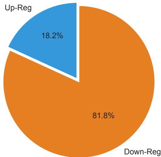
Directionality of V_g
