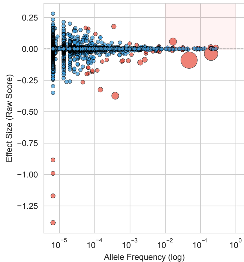
Purifying Selection (N=4665 vars)
