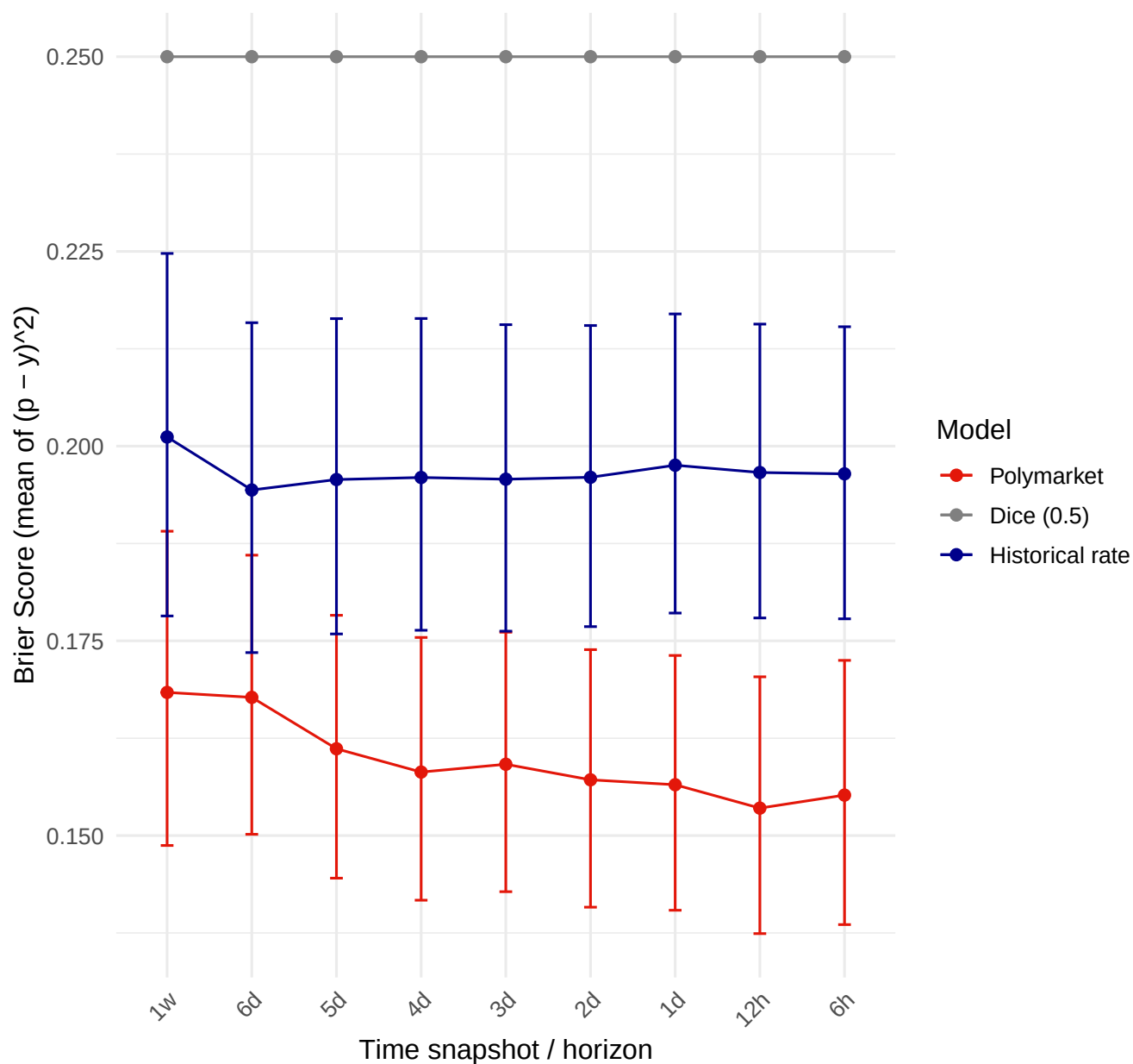
Brier Score by Time Horizon (with 95% CI)
