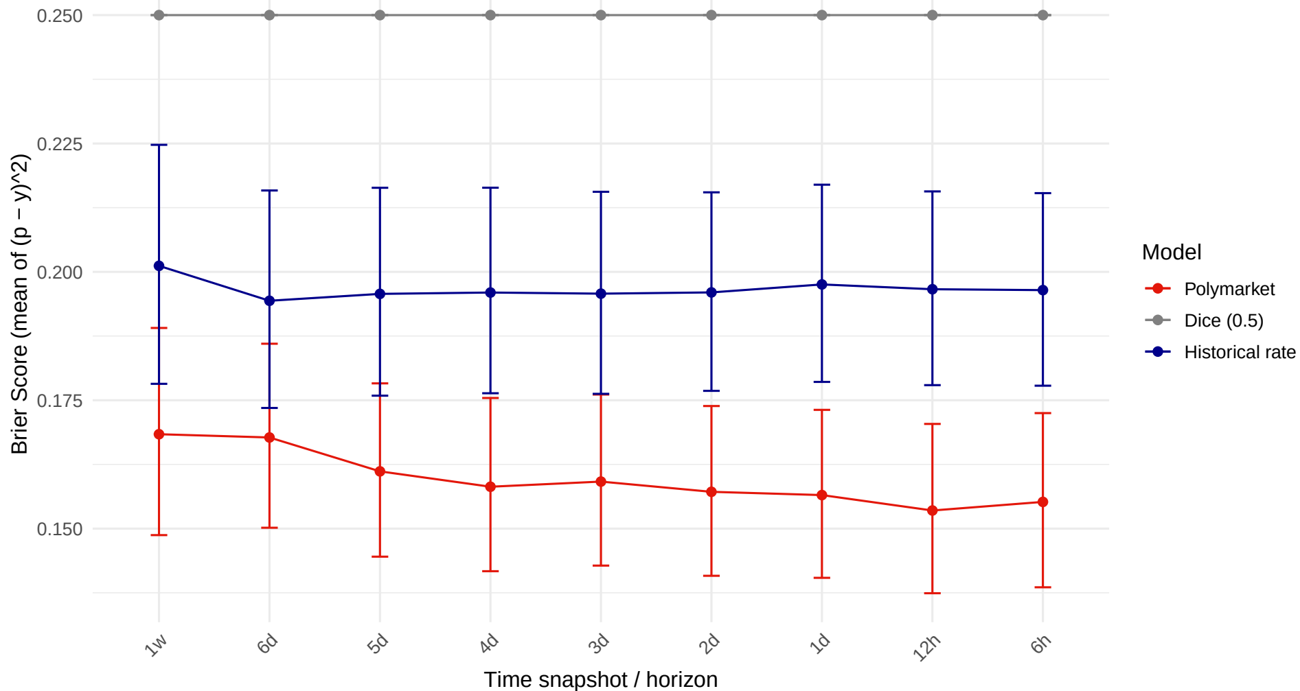
Brier Score by Time Horizon (with 95% CI)
