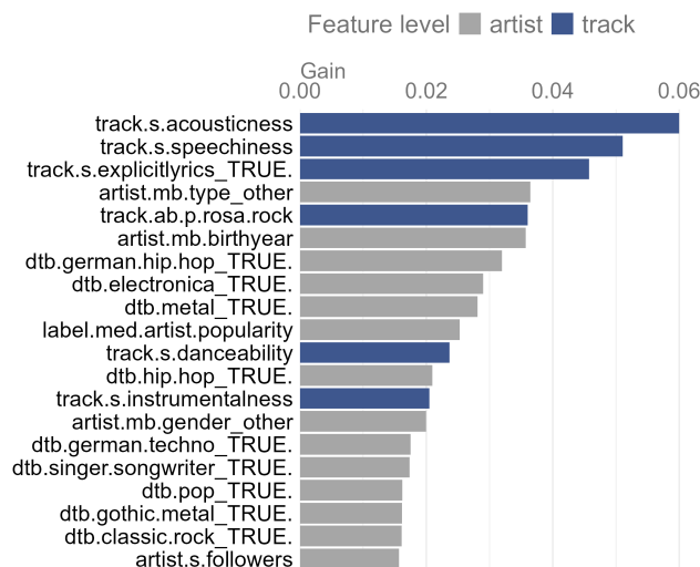
Figure 7: Top 20 most important features for automated classification of COMGET-5 with final LightGBM learner.
