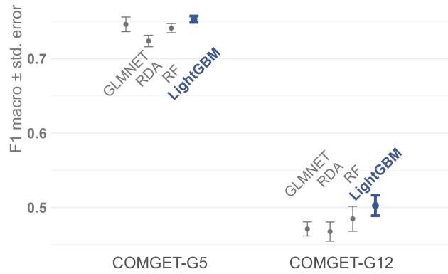
Figure 5: Performance comparison of different learners (GLMNET, RDA, RF, GBM) on 20% of the data set for low and medium genre granularity; plots show mean and standard error of F1_{macro} across CV folds.
