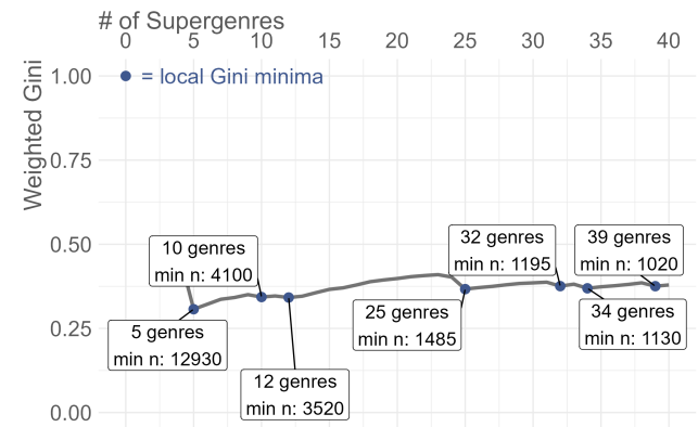
Figure 2: Within-hierarchy-level uniformity of distribution (weighted Gini coefficient, [0-1]) for different minimum song per genre counts when folding COMGET (searched in steps of 5 from 1,000 to 15,000).
