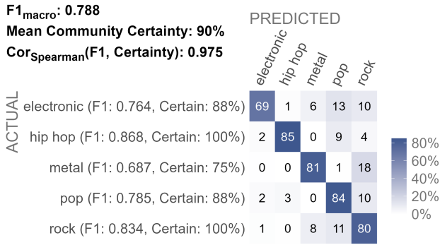
Figure 6: Confusion matrix for the final GBM model on the hold-out set for COMGET-5; grading shows P(\text{Predicted}|\text{Actual}) ; certainty is mean relative frequency of assignments within tracks that were assigned to the genre.
