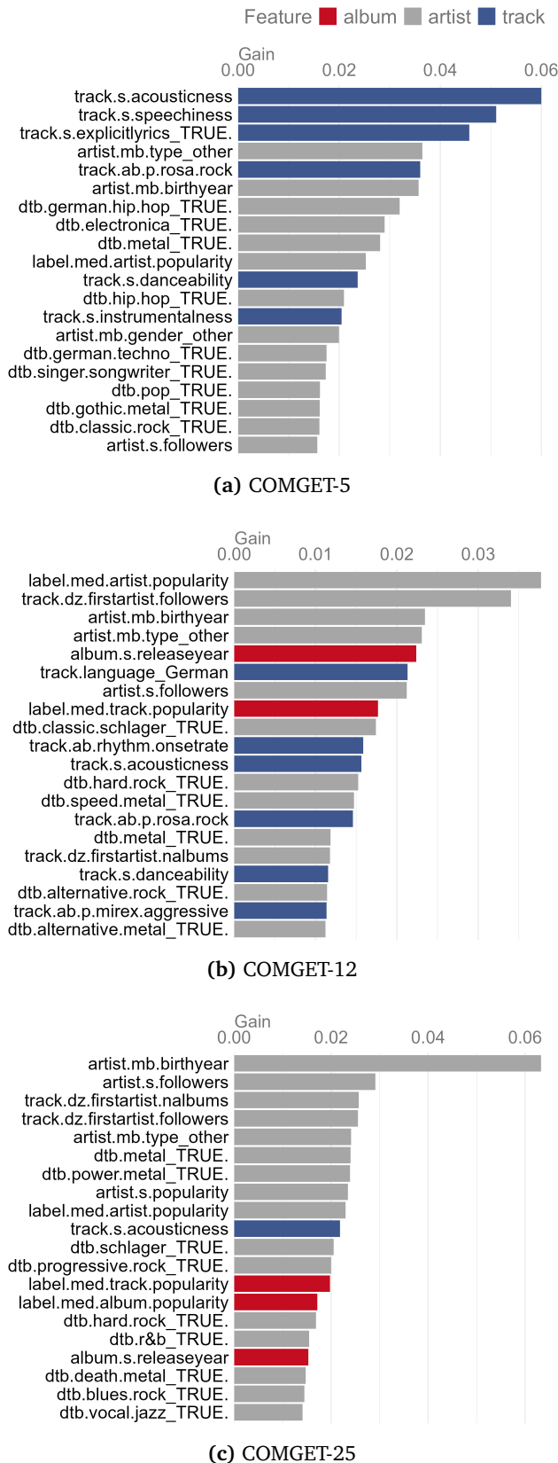
Figure 8: Top 20 most important features for automated classification of COMGET-5, COMGET-12, and COMGET-25 with final LightGBM learner.
