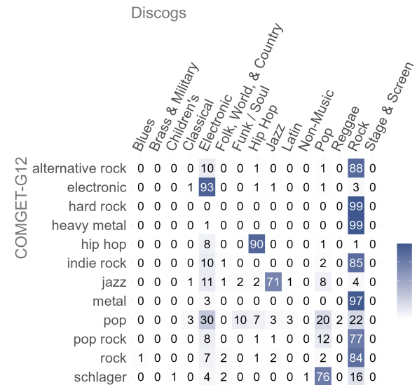
Figure 4: Contingency table comparing COMGET-G12 and Discogs genre assignments; values show P(\text{Discogs} | \text{COMGET-G12}) .
