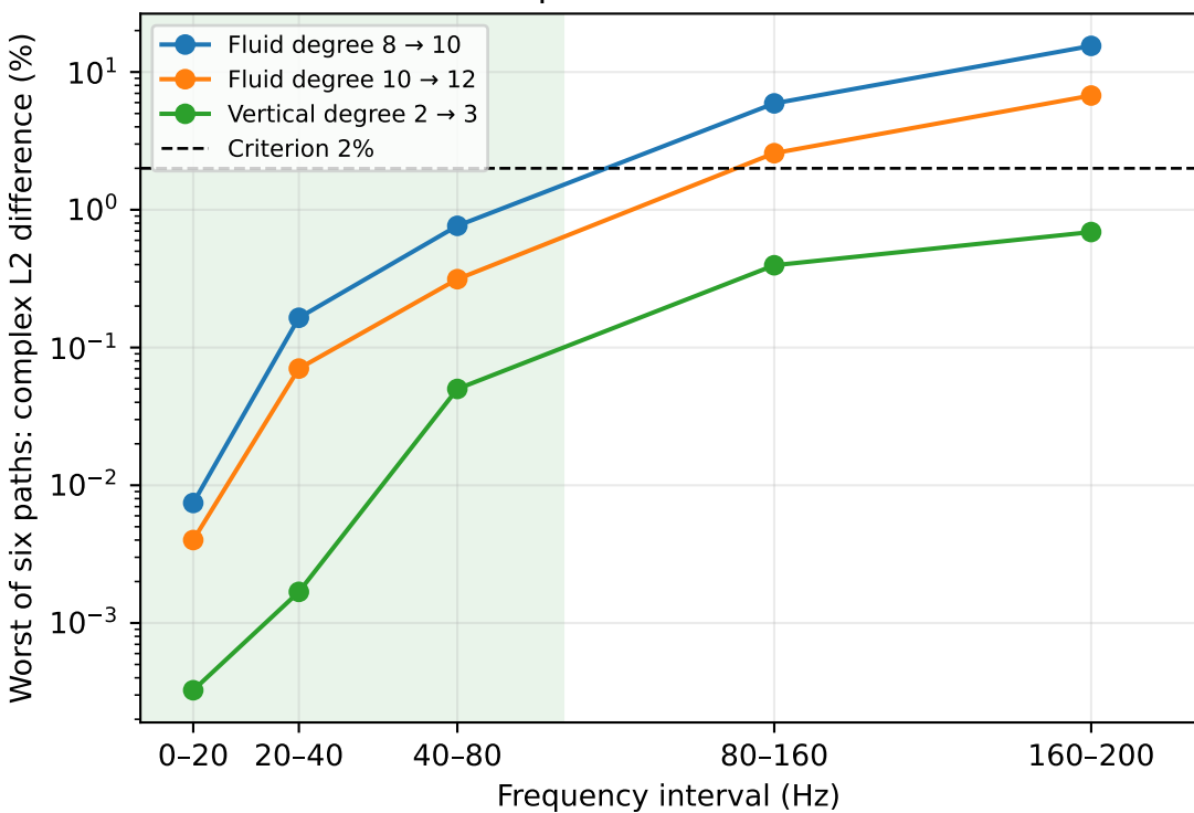
Fluid pressure refinement
