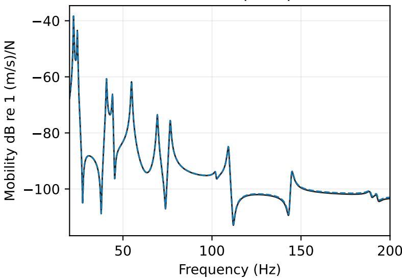
Exciter 1 → pickup 2
