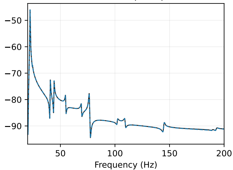
Exciter 3 → pickup 2
