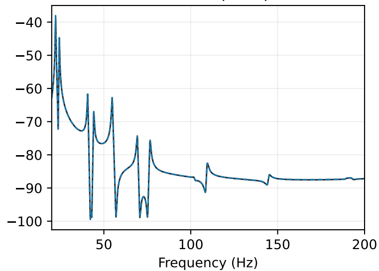
Exciter 2 → pickup 2
