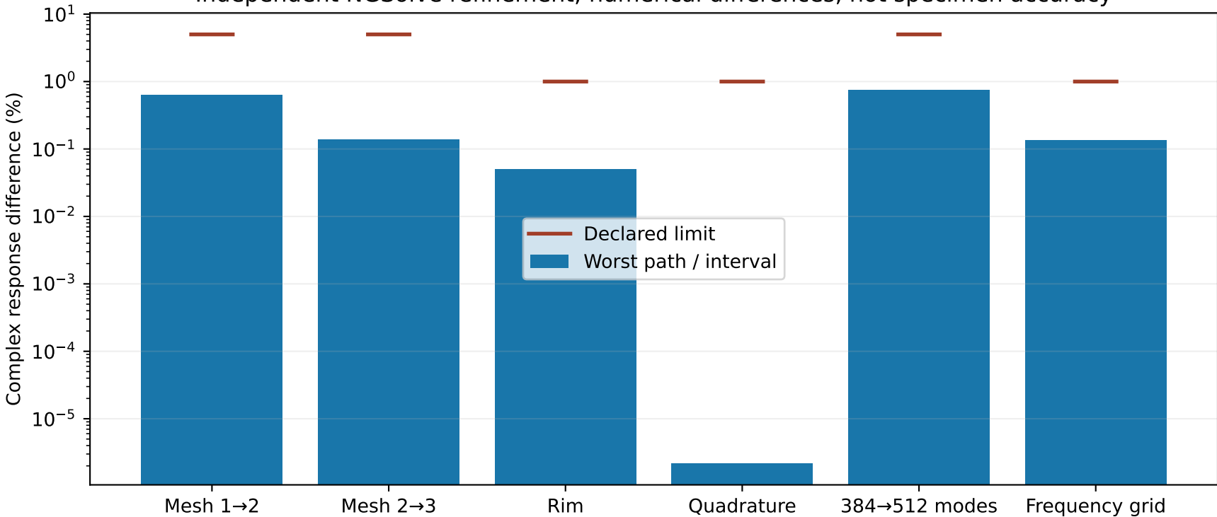
Independent NGSolve refinement; numerical differences, not specimen accuracy
