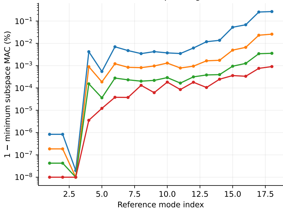
Vector-mode/subspace agreement
