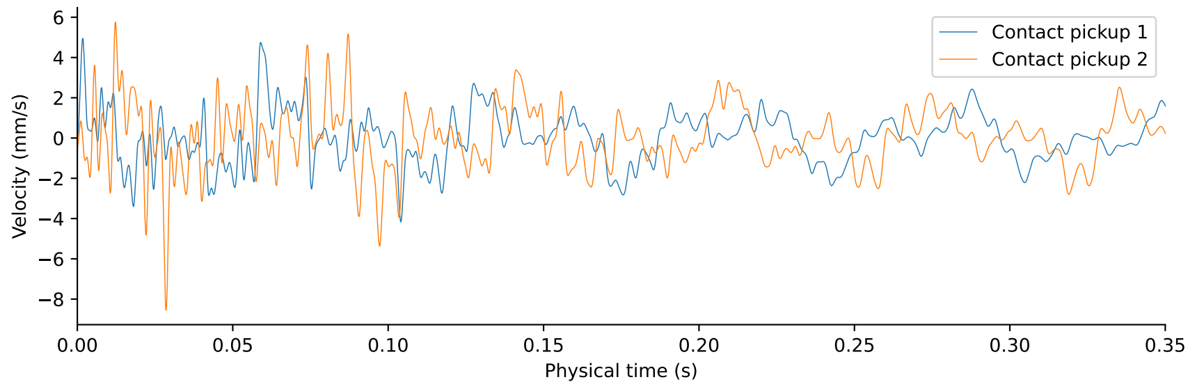
Finite-patch impulse response; two point pickups and retained energy
