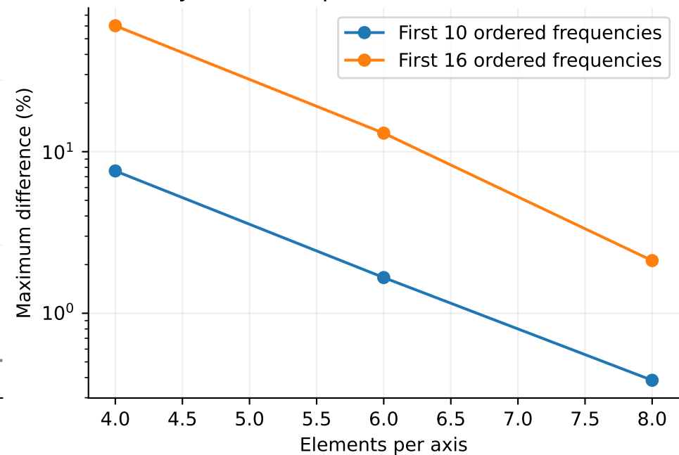
Dry basin: comparison with 10 \times 10 cells
