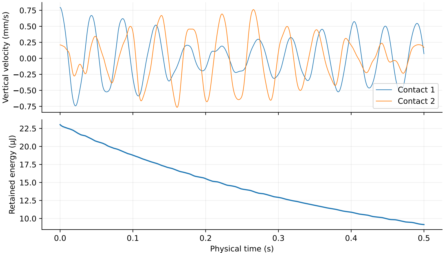
Default impulse: retained dry-shell response
