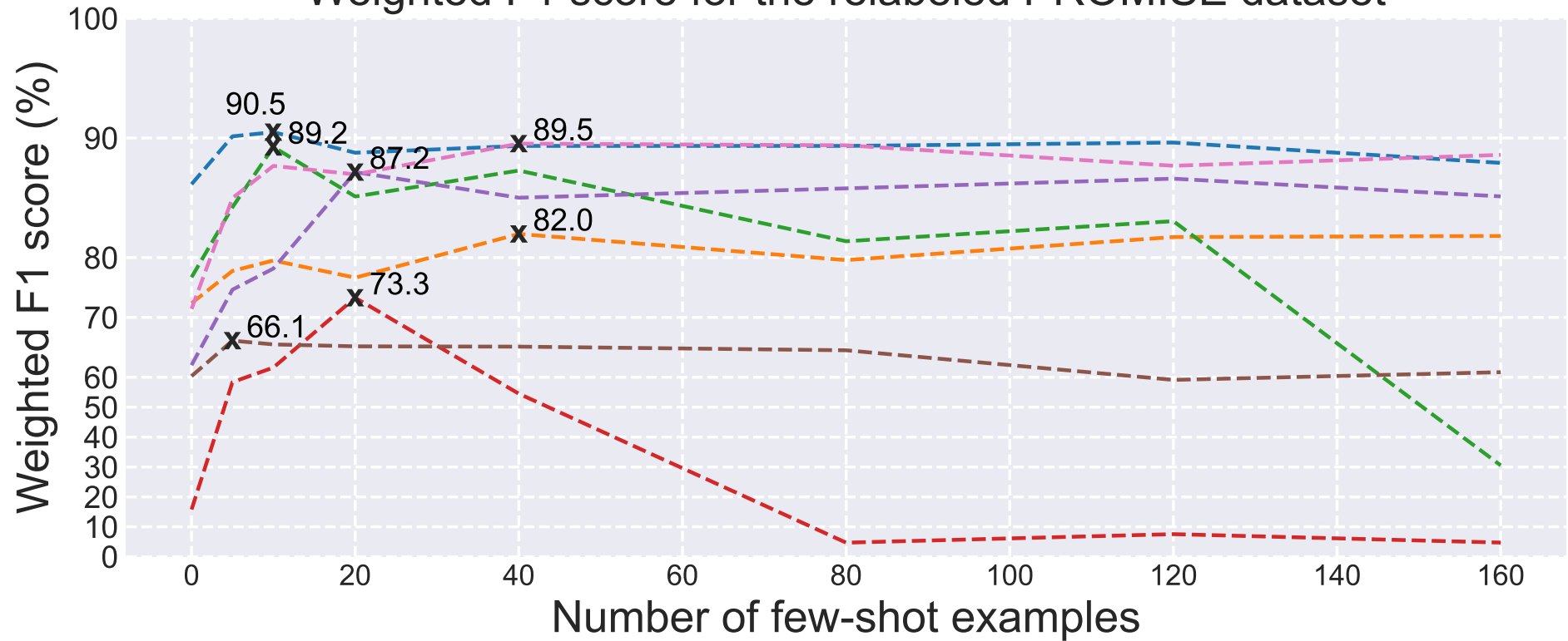
Weighted F1 score for the relabeled PROMISE dataset
