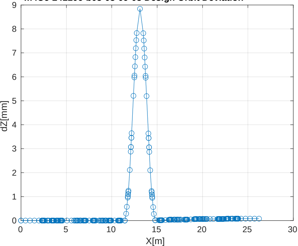
m4Uc-241106-b03-03-09-08 Design Orbit Deviation
