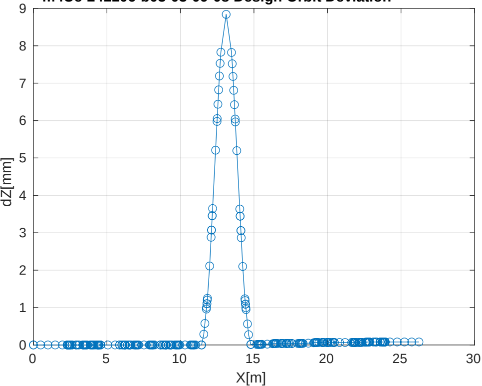
m4Uc-241106-b03-03-09-08 Design Orbit Deviation
