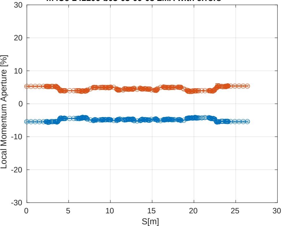
m4Uc-241106-b03-03-09-08 LMA with errors
