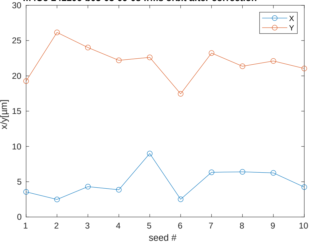
m4Uc-241106-b03-03-09-08 :rms orbit after correction
