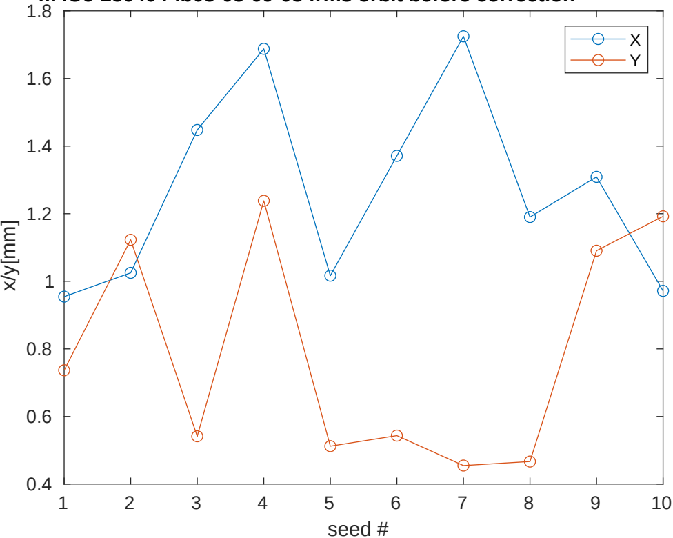
m4Uc-250404-ib03-03-09-08 :rms orbit before correction
