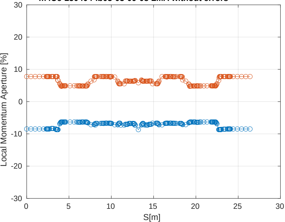
m4Uc-250404-ib03-03-09-08 LMA without errors
