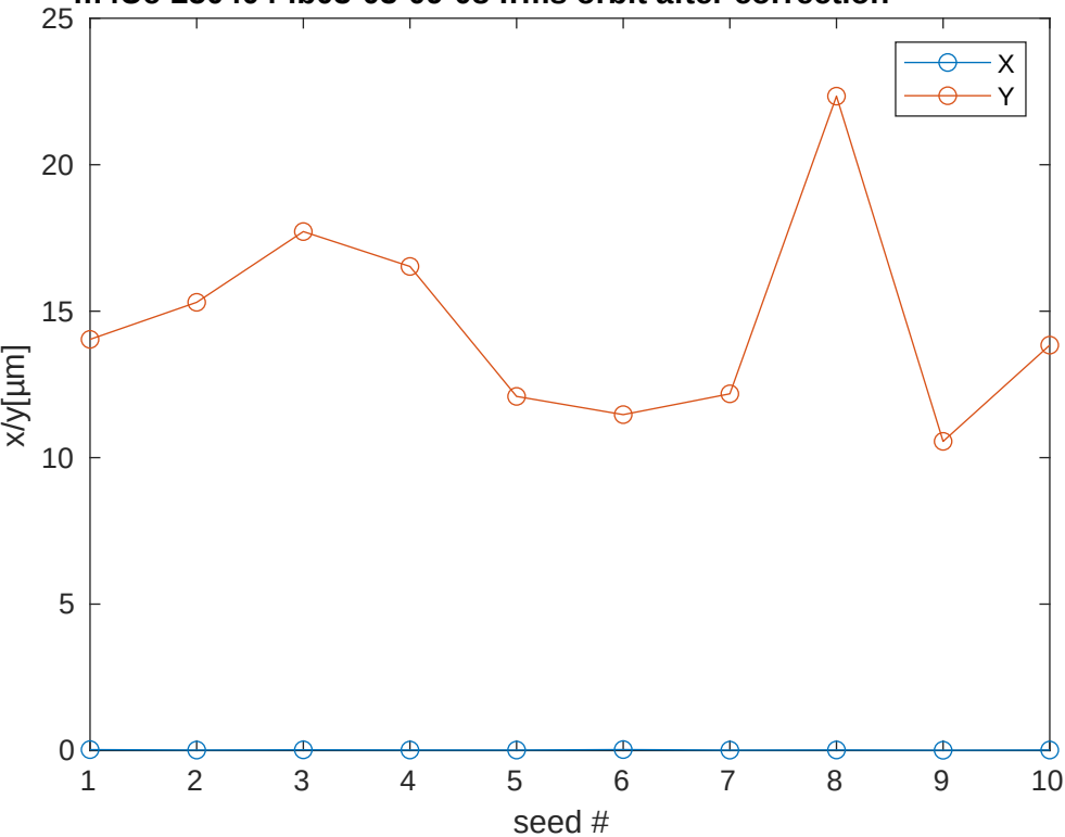
m4Uc-250404-ib03-03-09-08 :rms orbit after correction
