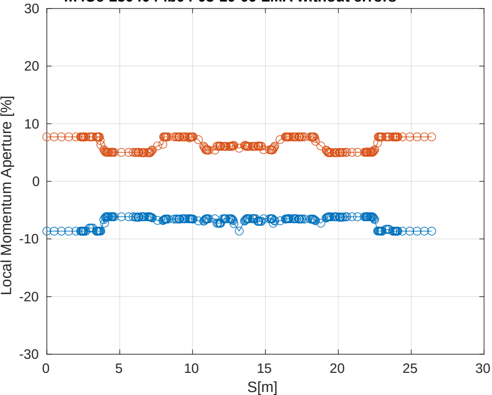
m4Uc-250404-ib04-03-10-09 LMA without errors
