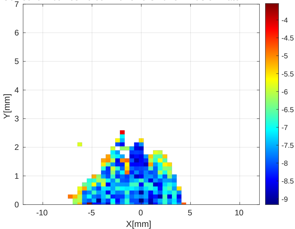
m4Uc-250404-ib04-03-10-09: with errors Tune Diffusion Rate
