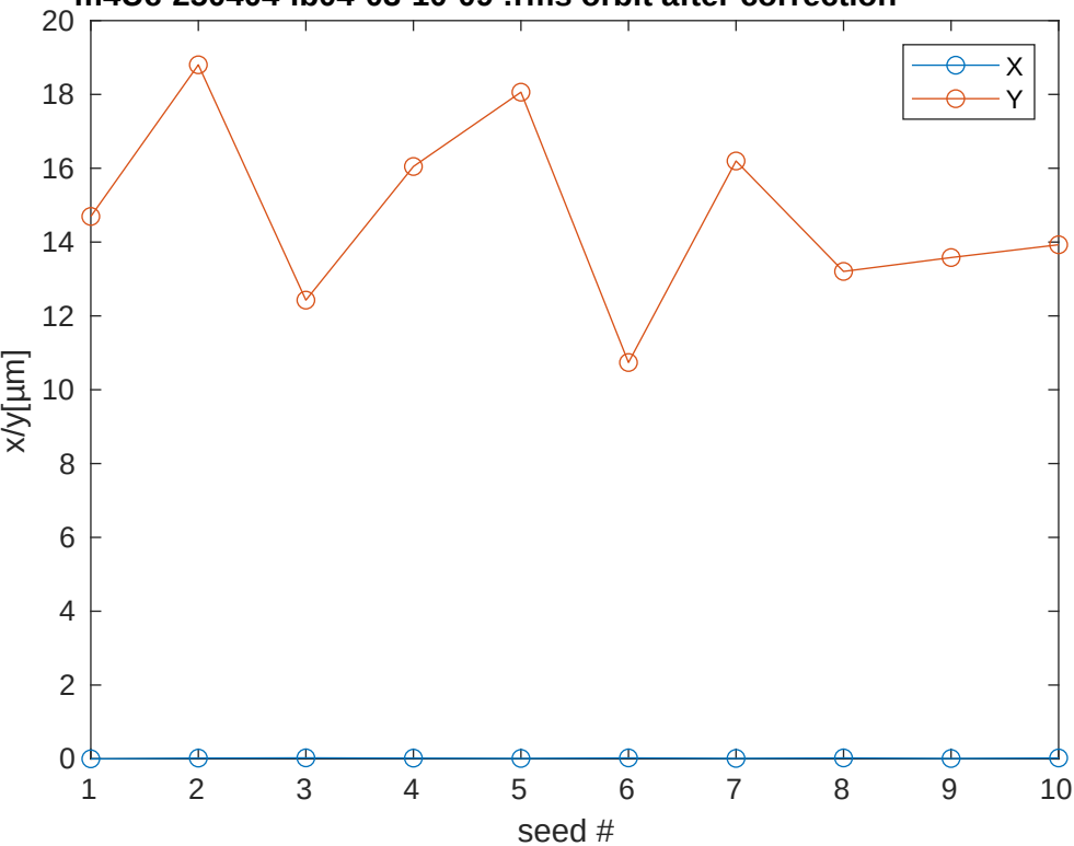
m4Uc-250404-ib04-03-10-09 :rms orbit after correction
