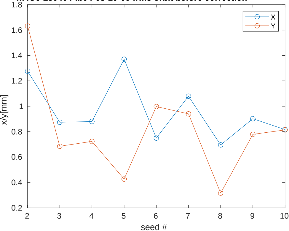
m4Uc-250404-ib04-03-10-09 :rms orbit before correction
