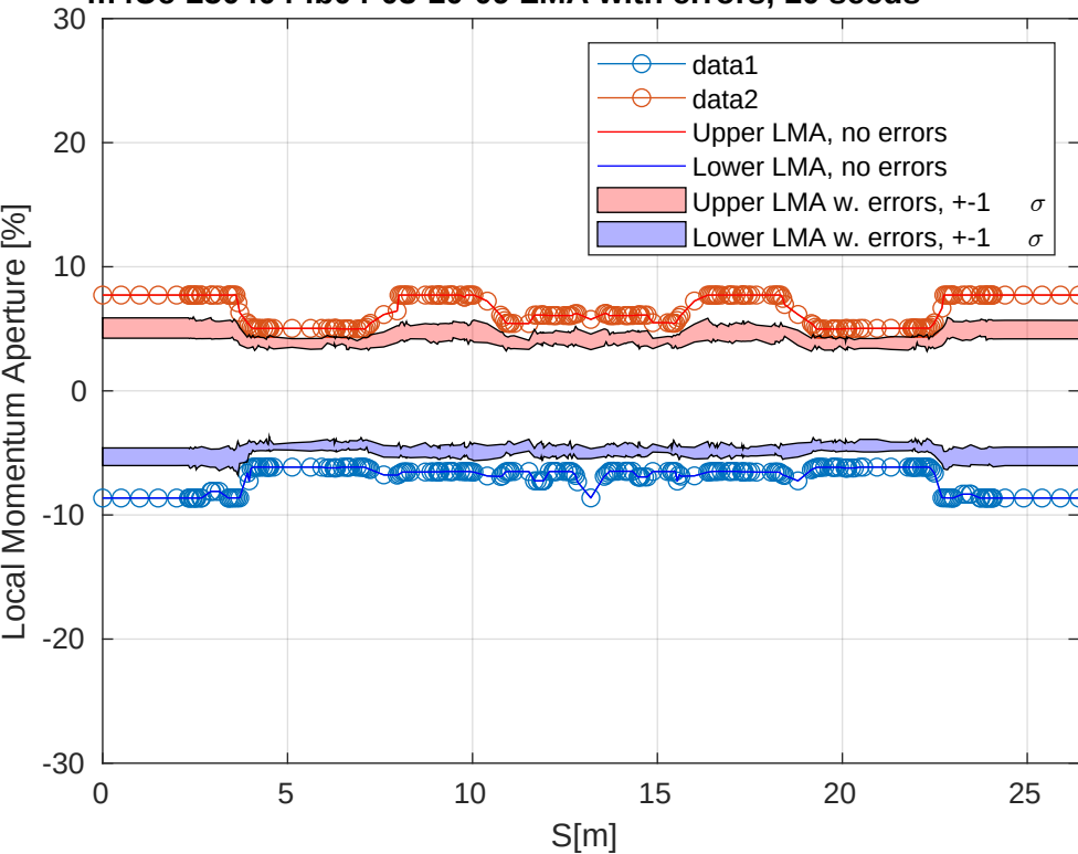
m4Uc-250404-ib04-03-10-09 LMA with errors, 10 seeds
