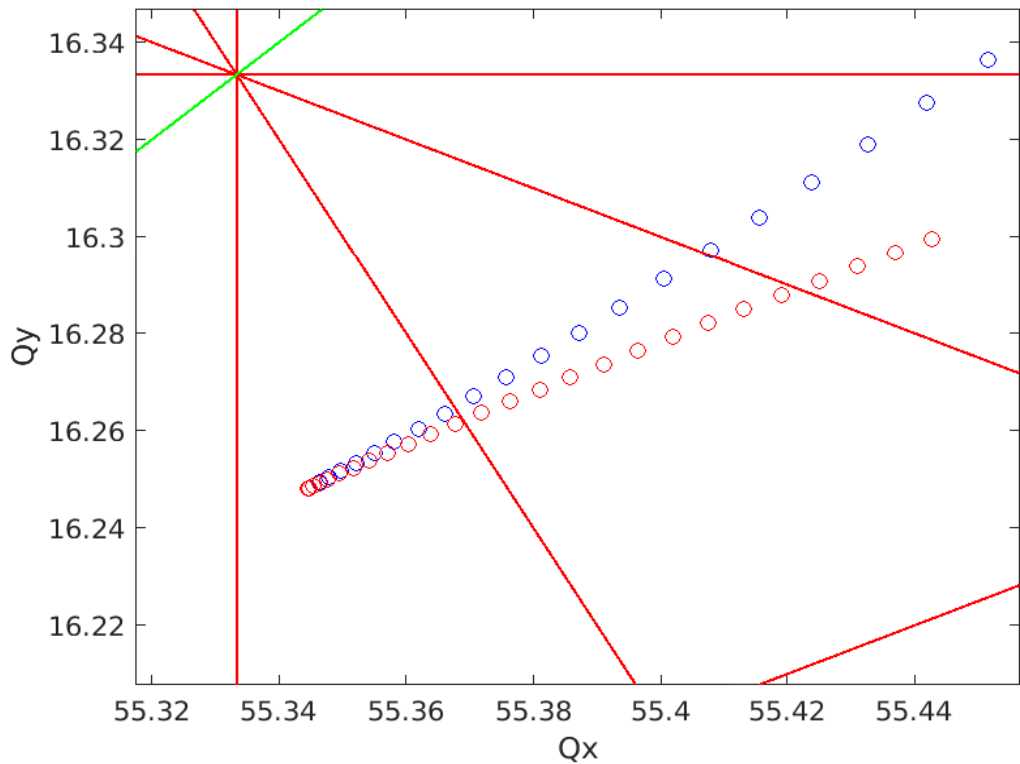
m4Uc-250404-ib04-03-10-09 chrom=0 Res order=3
