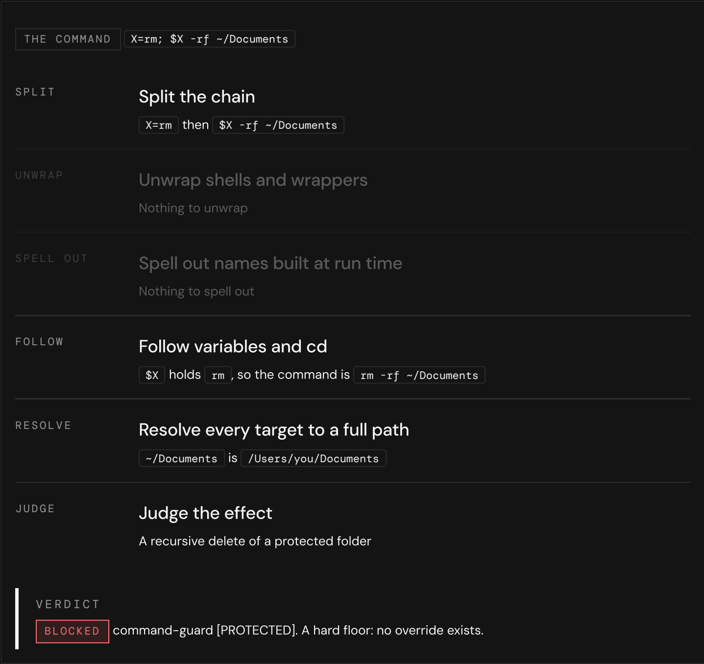
Figure 2 · The stages command-guard's code goes through, one per line. The code runs them interleaved, and again inside every nested command. Each verdict is its real output on 2 Oct 2026.
