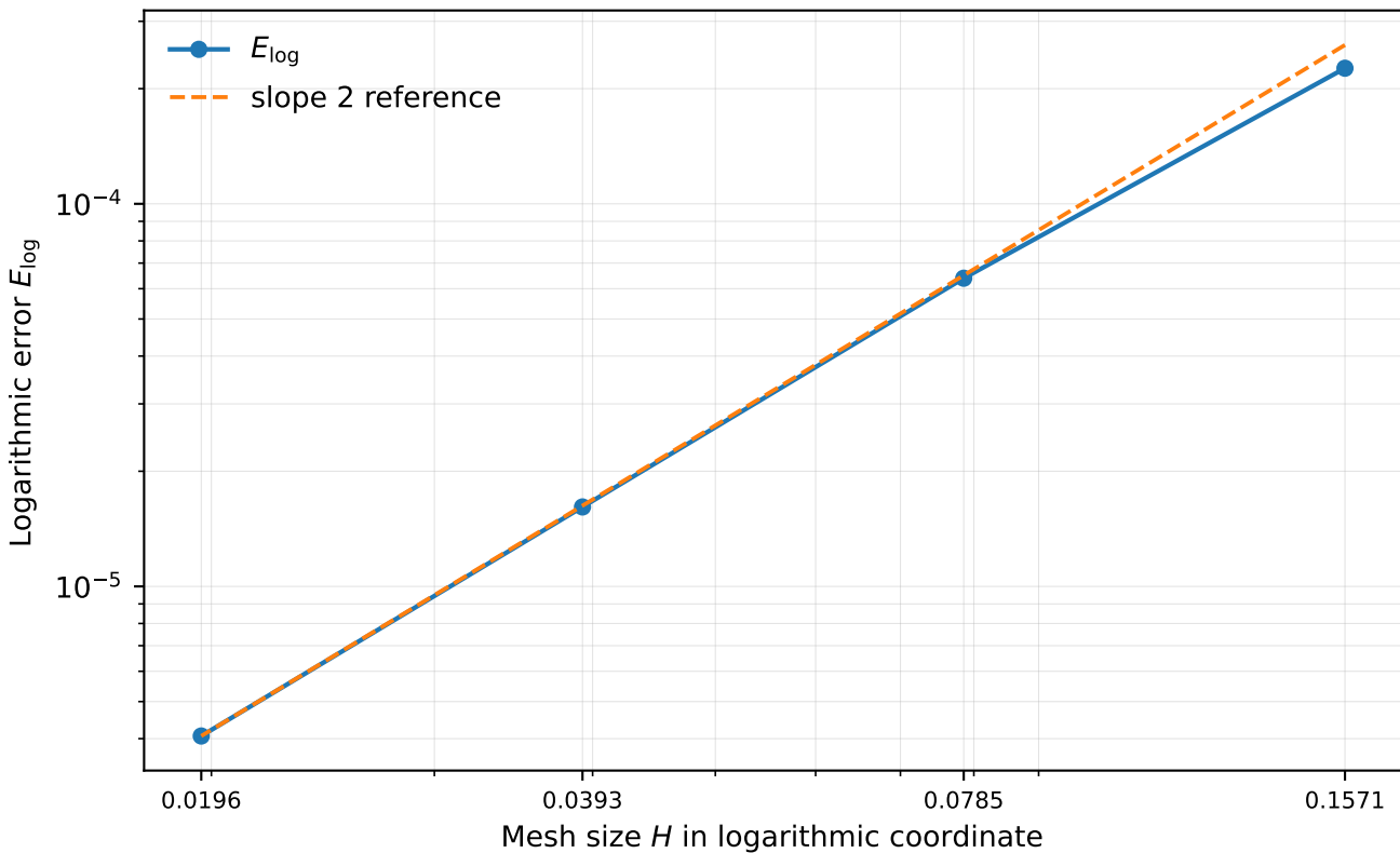
Second-order convergence in logarithmic maximum norm
