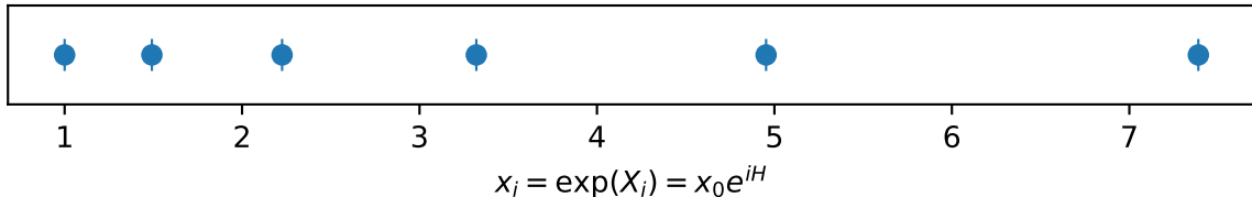
Induced geometric grid in the positive variable
