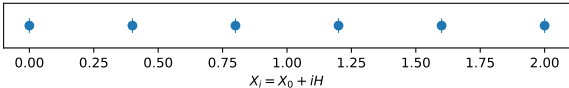
Uniform grid in logarithmic coordinate
