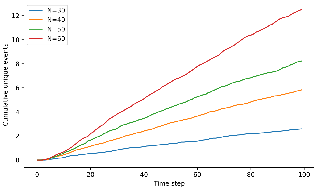
Temporal evolution by swarm size, \rho=4.55 , smallest domain
