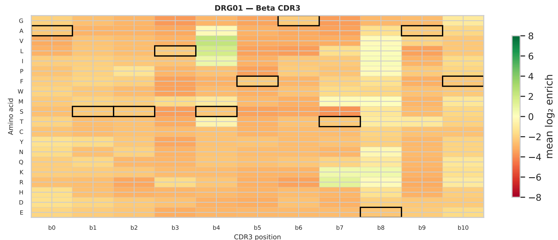
Residue enrichment per CDR3 position (mean log 2 enrichment, all variants)
