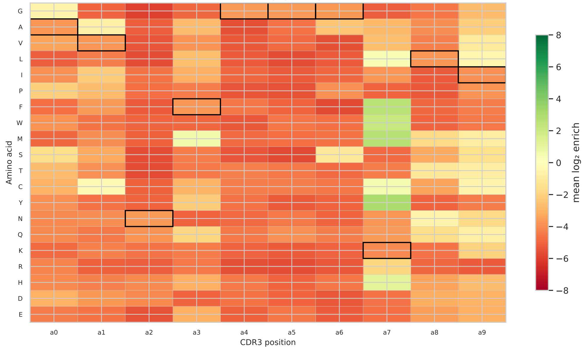
Alpha CDR3 — all peptides pooled
