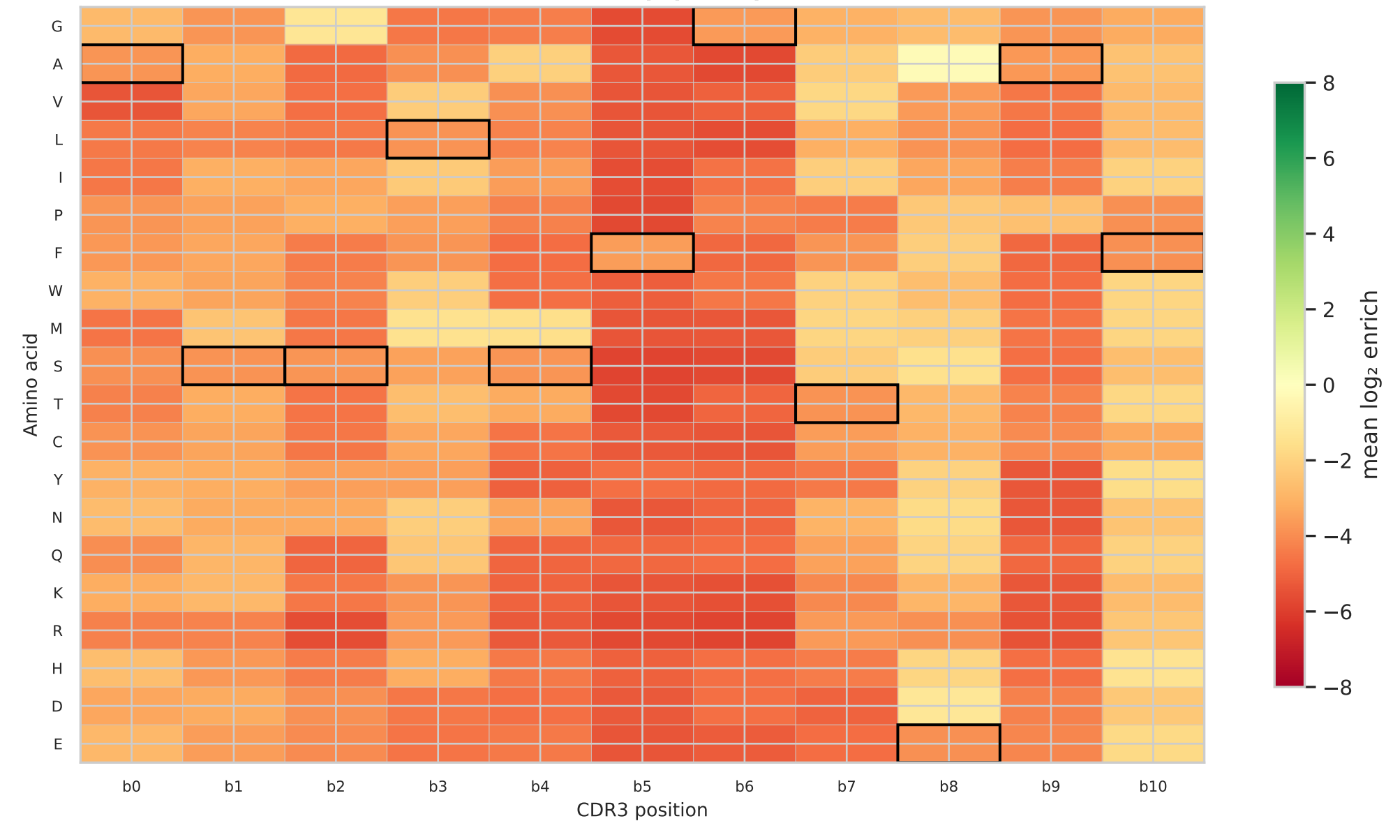
Beta CDR3 — all peptides pooled
