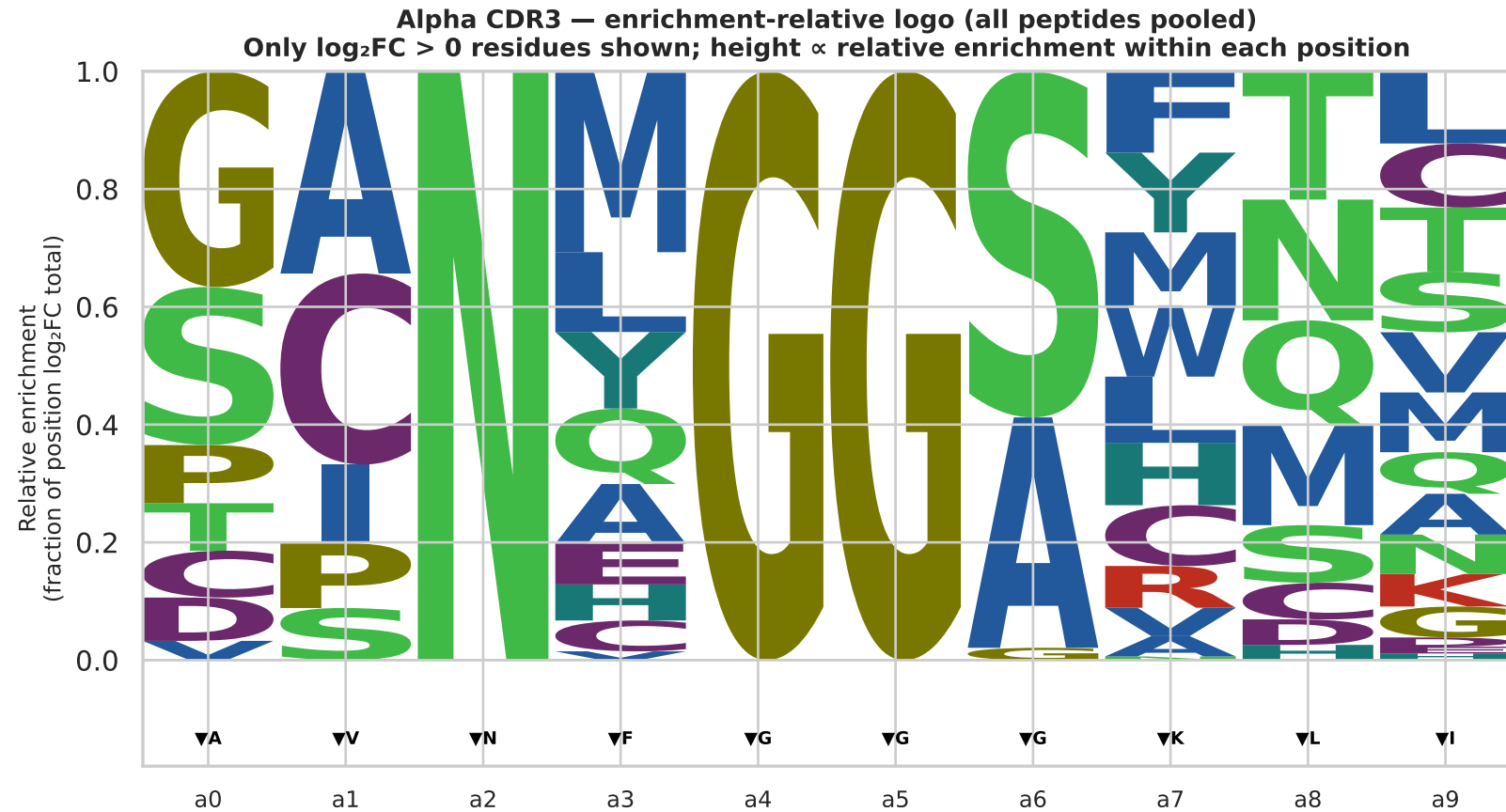
Enrichment-relative sequence logoplots — all peptides pooled Score: \log_2[ P(\text{enriched} \mid \text{aa at pos}) / \text{global baseline} ] · Normalized within each position so heights sum to 1
