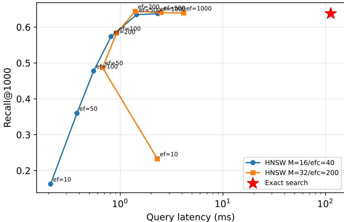
ANN speed-recall tradeoff, GTE-large, 400K tier
