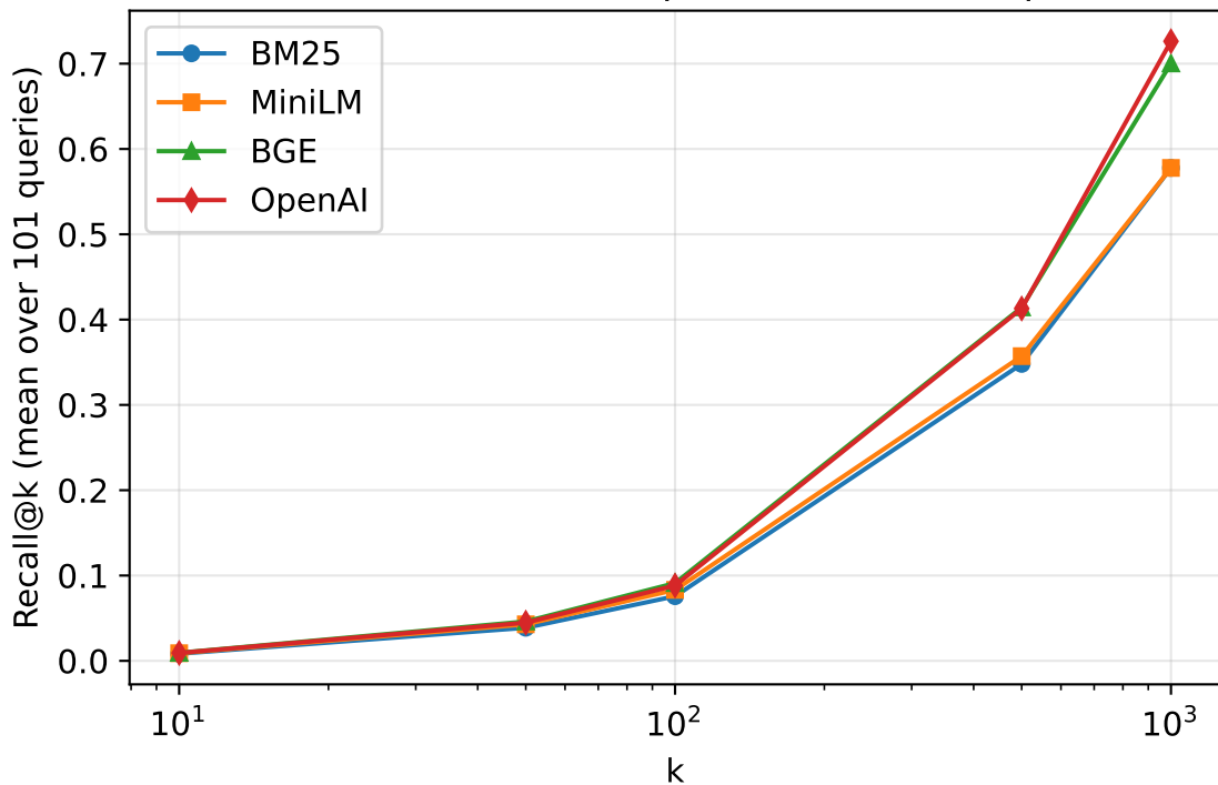
Baseline Recall@k, strict pseudo-relevance protocol
