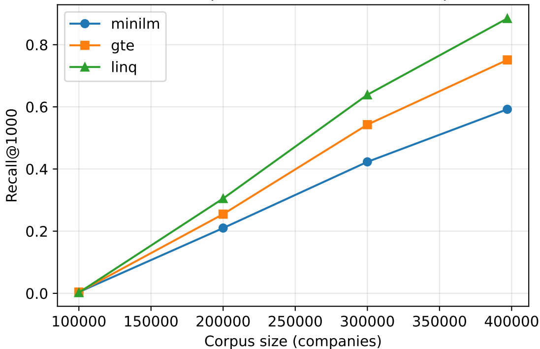
Production-independent test: recall vs. corpus size
