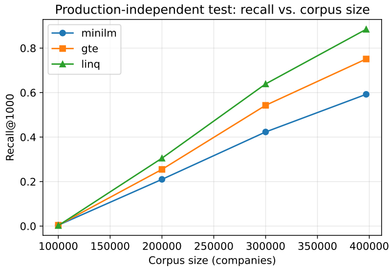
Figure 5.1: Recall@1,000 against the production-independent relevant set, as a function of corpus size, for all three retrieval methods evaluated.
