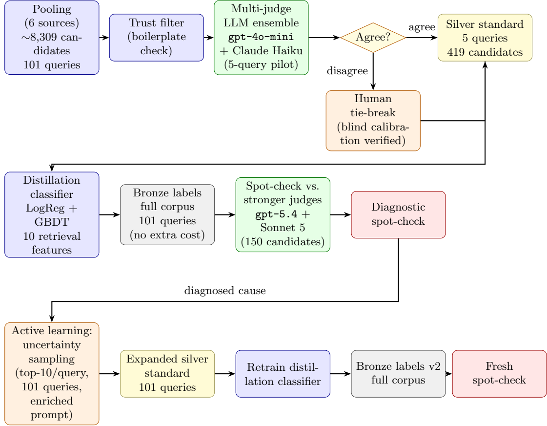
Figure 4.2: The silver and bronze standard construction pipeline, from pooling through active-learning expansion.
