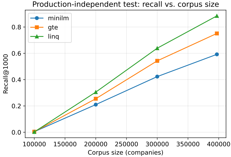
Figure 5.1: Recall@1,000 against the production-independent relevant set, as a function of corpus size, for all three retrieval methods evaluated.
