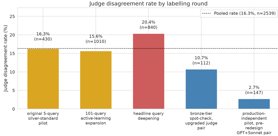
Figure 4.1: Judge disagreement rate by labelling round. The dashed line marks the pooled rate across all 2,539 doubly-judged candidates.
