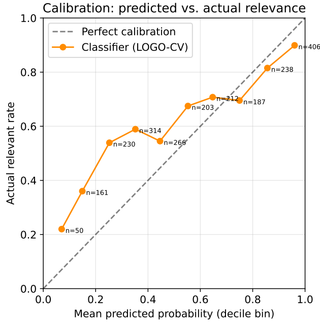
Figure 5.2: Calibration reliability diagram: mean predicted probability vs. actual relevant rate per decile bin, against the diagonal of perfect calibration.
