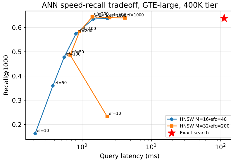
Figure 5.3: ANN speed-recall tradeoff at the 400K tier (GTE-large): Recall@1,000 vs. query latency across the ef_search sweep, both build configurations, against the exact-search reference point.
