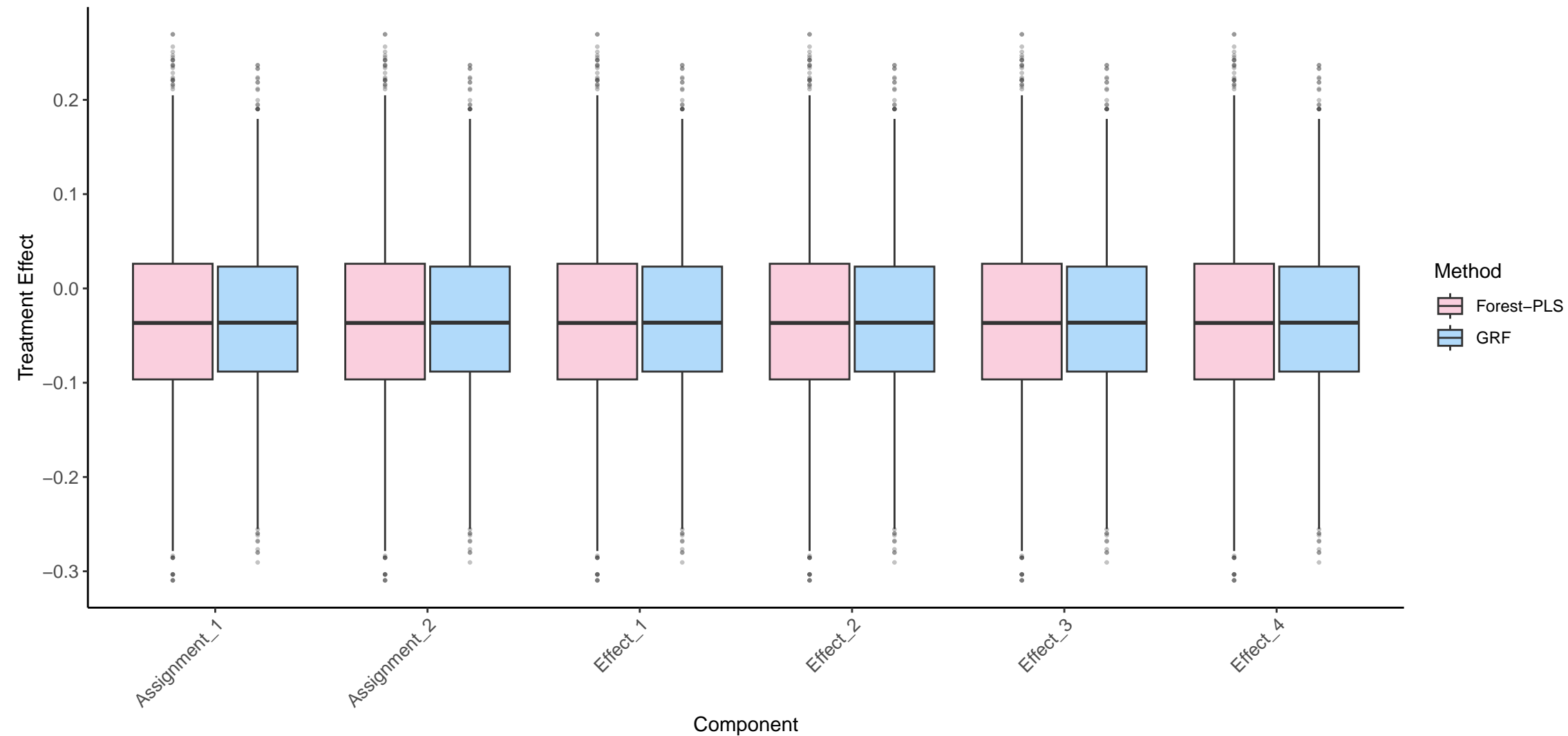
Treatment Effect Distribution by Component
