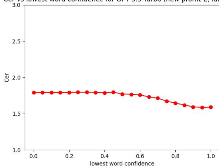
Cer vs lowest word confidence for GPT-3.5-Turbo (new prompt-2, large-v3)
