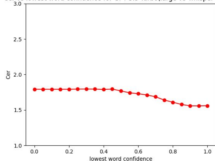
Cer vs lowest word confidence for GPT-3.5-Turbo(large-v3 whisper model)
