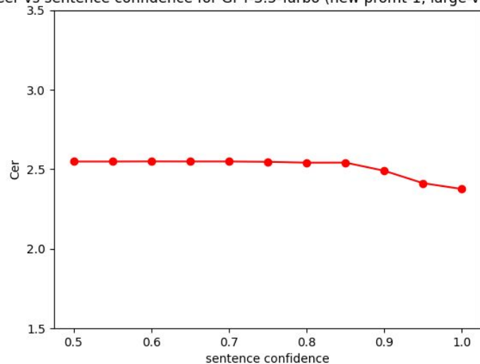
Cer vs sentence confidence for GPT-3.5-Turbo (new prompt-1, large-v3, noisy)
