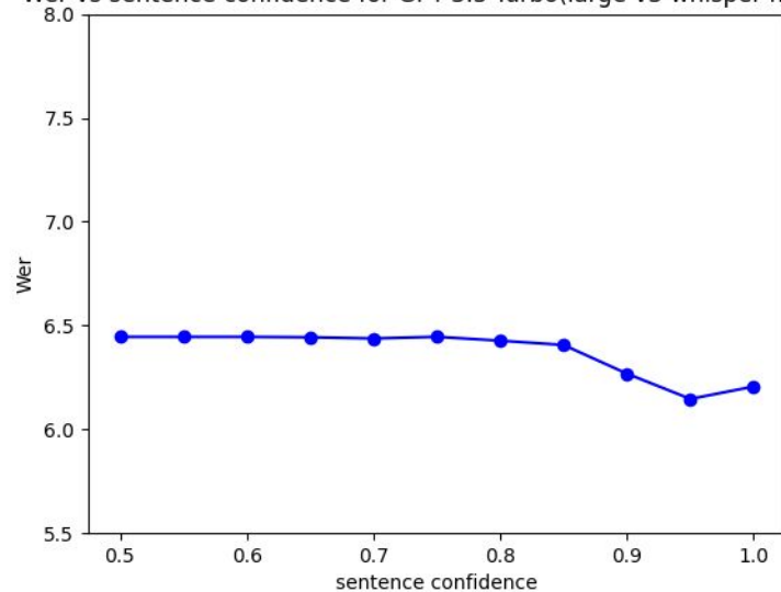
Wer vs sentence confidence for GPT-3.5-Turbo(large-v3 whisper model)
