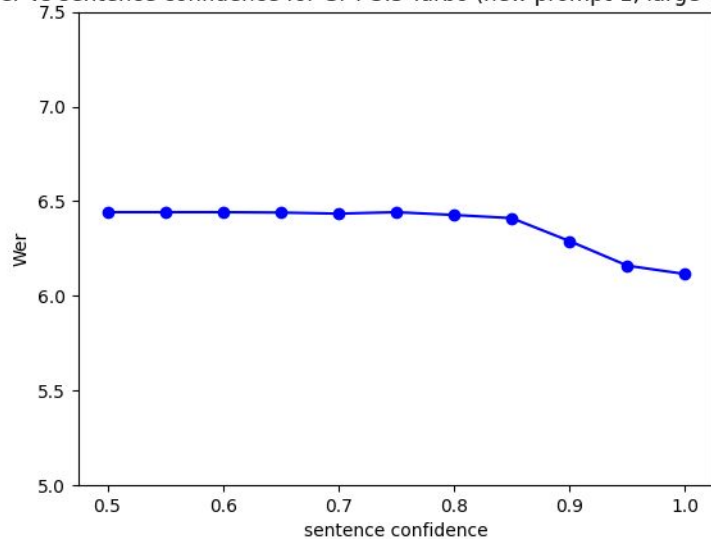
Wer vs sentence confidence for GPT-3.5-Turbo (new prompt-1, large-v3, noisy)
