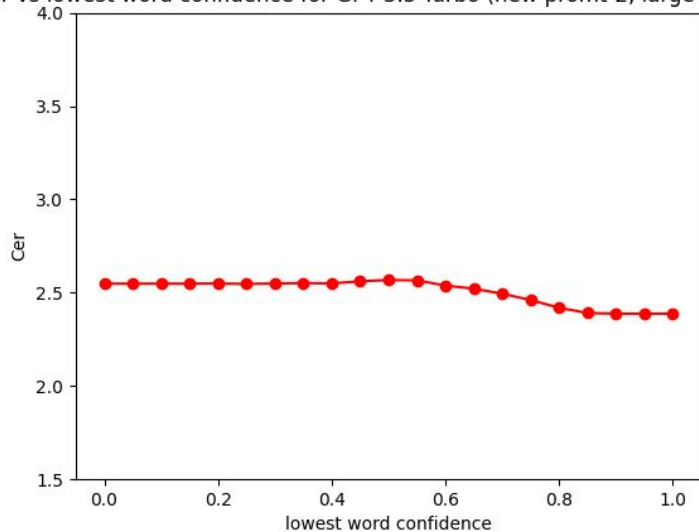
Cer vs lowest word confidence for GPT-3.5-Turbo (new prompt-2, large-v3, nois)
