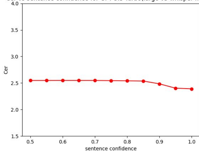
Cer vs sentence confidence for GPT-3.5-Turbo (large-v3 whisper model)
