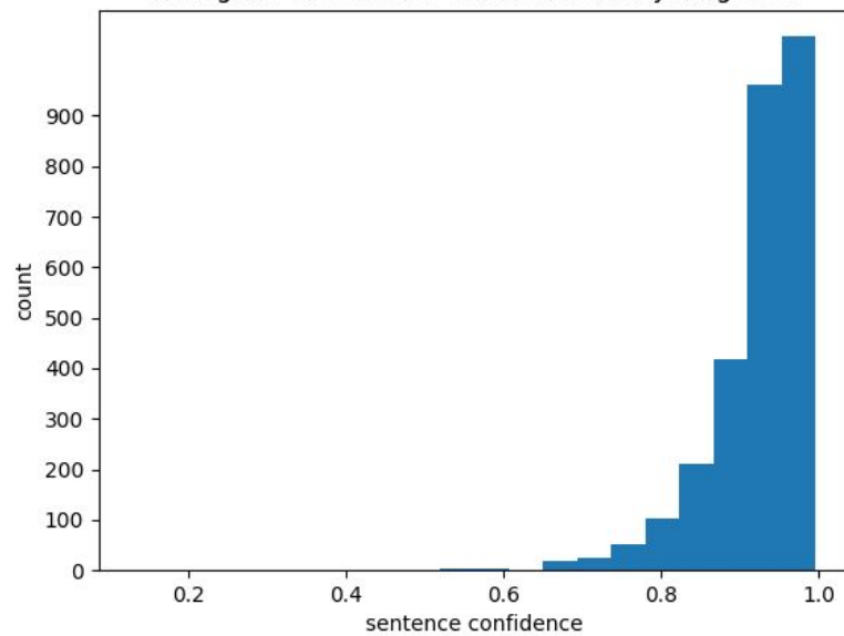
Histogram of sentence confidence (noisy, large-v3)
