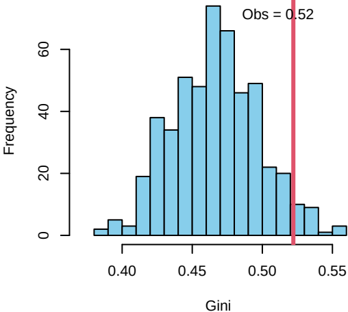
Gini (in-strength)
