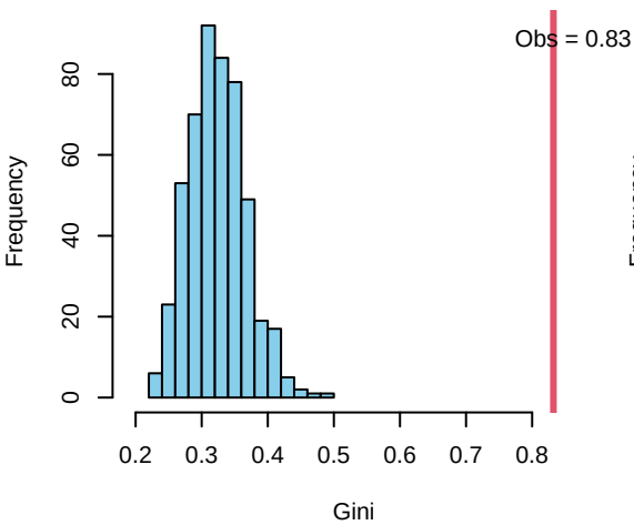
Gini (in-strength)
