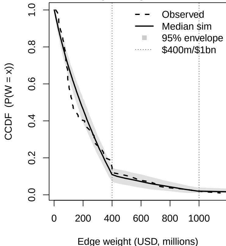
Edge-weight CCDF
