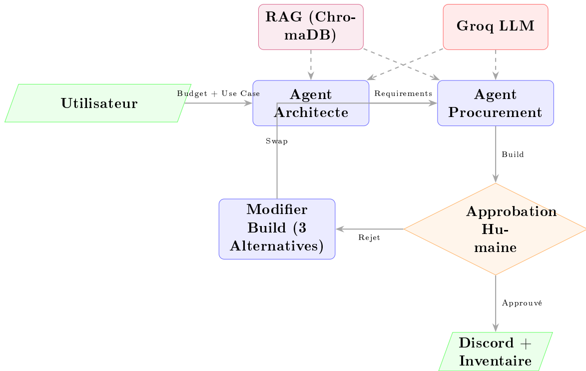
FIGURE 1 – Architecture globale du système multi-agent
