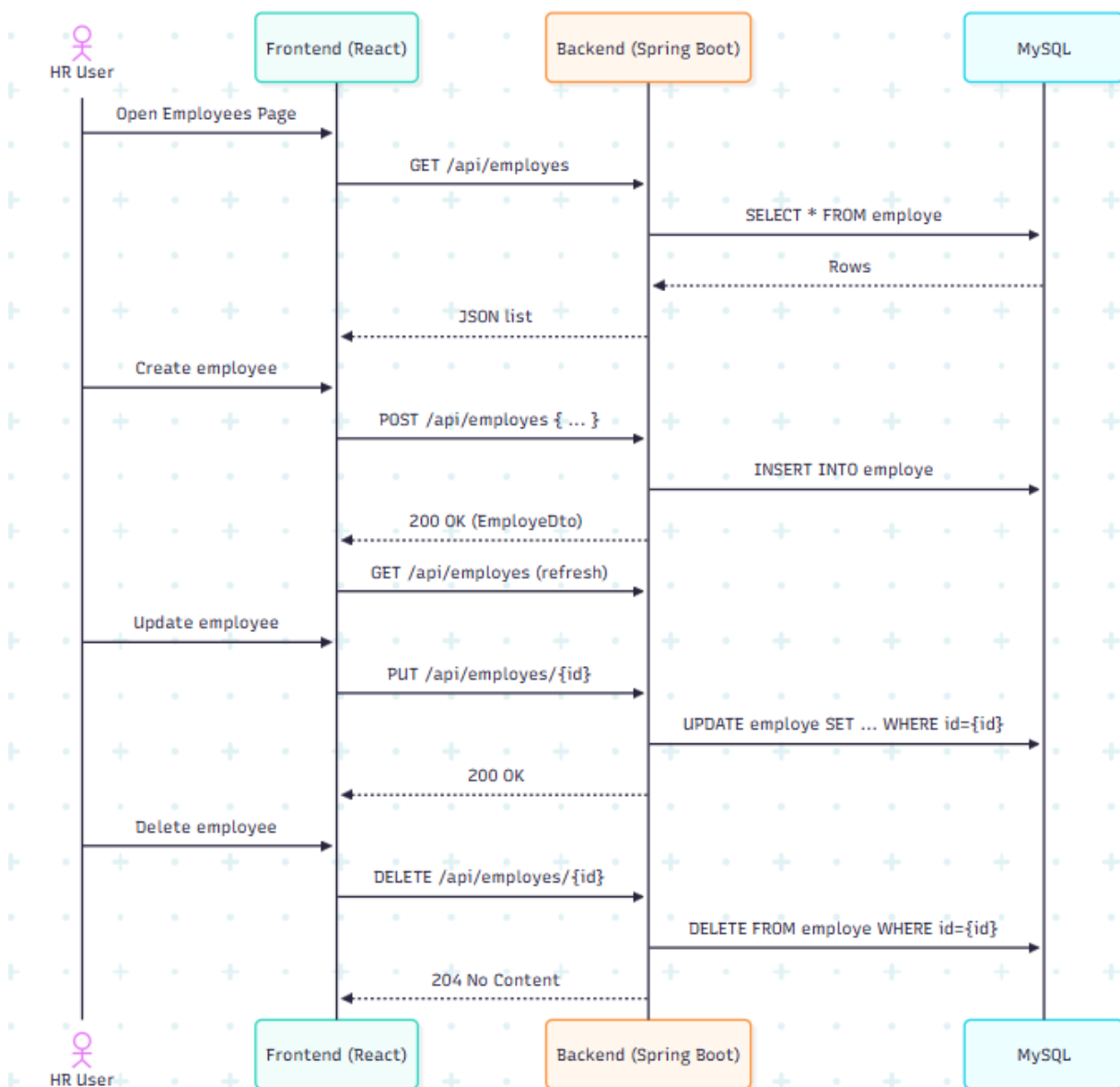
Figure 3.6: Sequence Diagram - Employee Management
