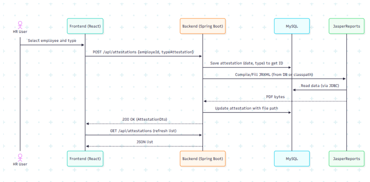
Figure 3.5: Sequence Diagram - Attestation Generation Process
