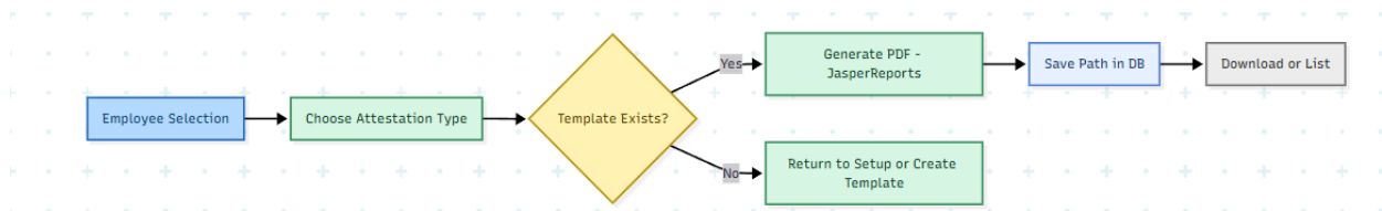
Figure 3.10: Attestation Generation Flow
