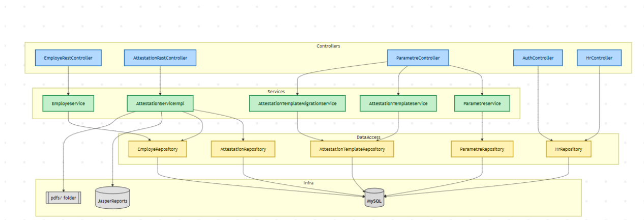
Figure 3.8: Backend Layered Architecture
