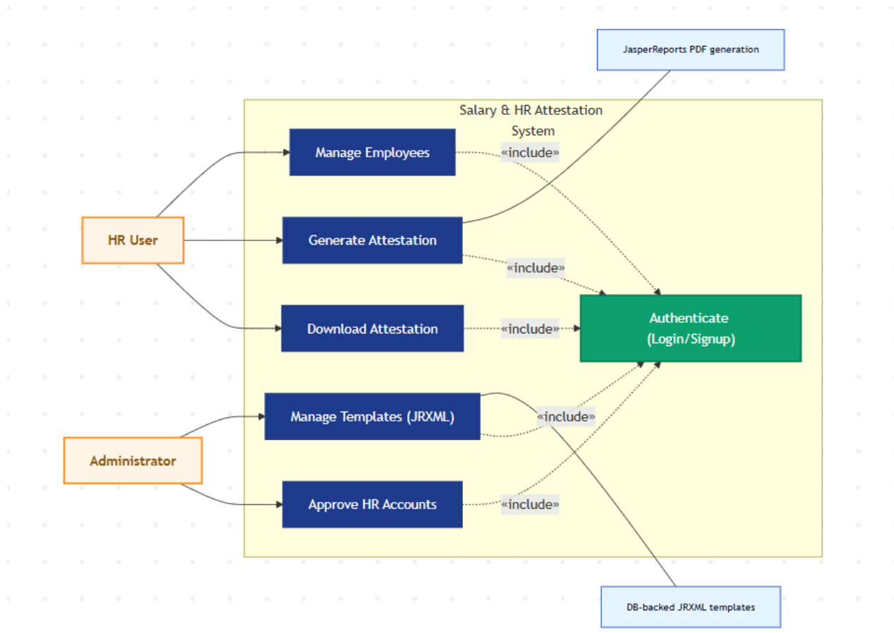
Figure 3.4: Use Case Diagram - System Actors and Interactions
