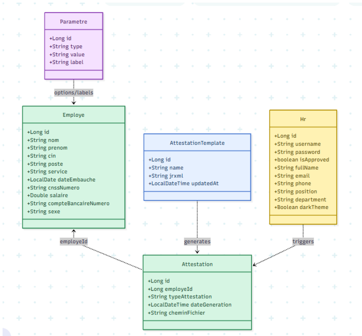
Figure 3.7: UML Class Diagram - Global Data Model
