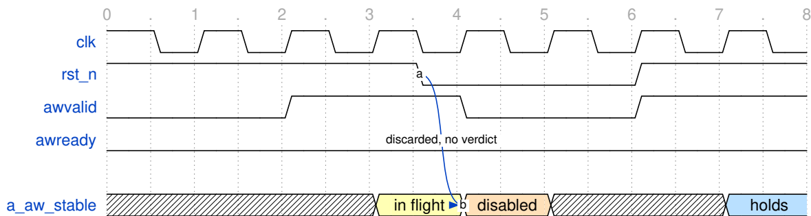
Figure 11.3 — Reset falls between cycles 3 and 4, discarding the in-flight attempt rather than judging it; the attempt after release at cycle 6 holds.
