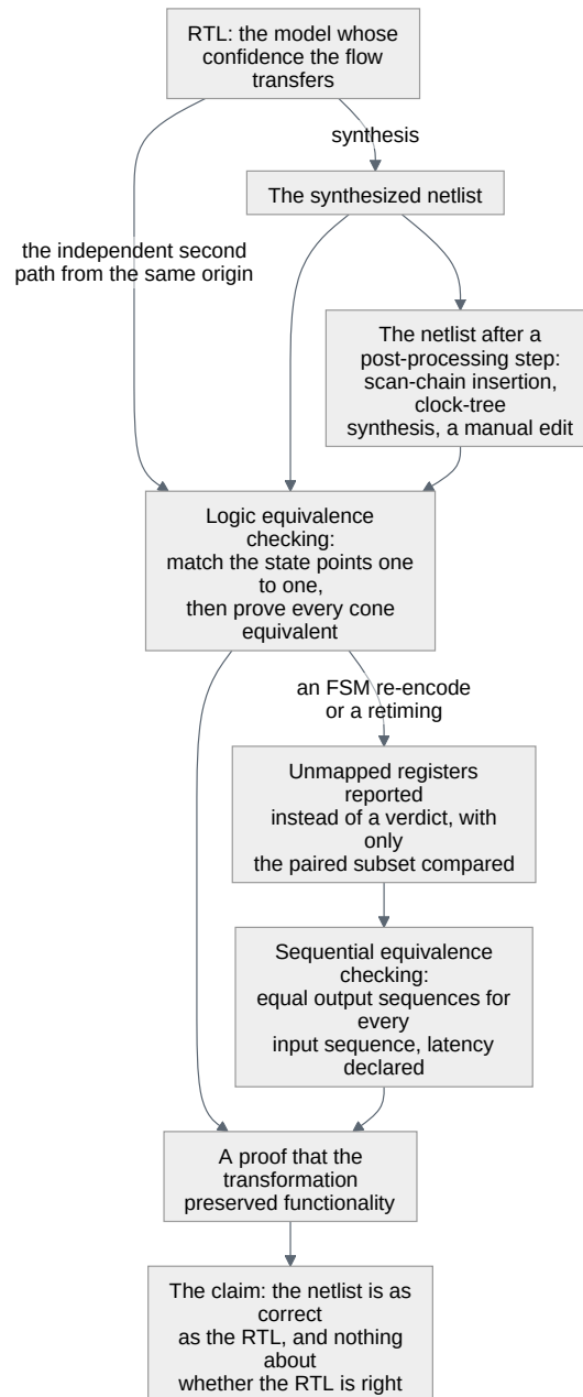
Figure 15.1 — Equivalence checking as a second path from the same origin: every transformation of the design owes one proof, a broken state-point mapping is what sends a step to the sequential flow, and the claim stays relative to the RTL.
