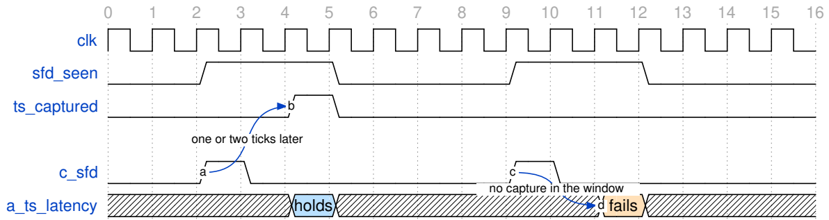
Figure 11.10 — Delimiter 2 captures at 4 inside the window; delimiter 9 has no capture by 11 and fails.
