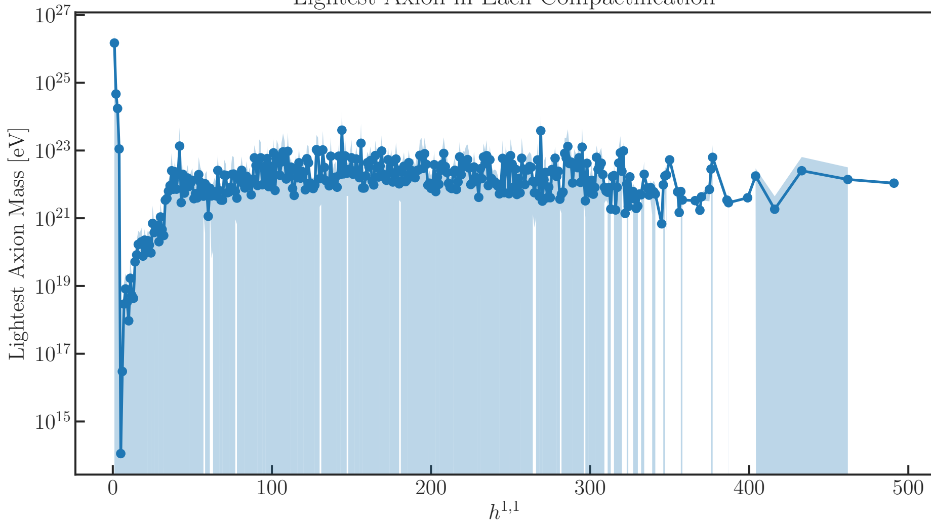
Lightest Axion in Each Compactification
