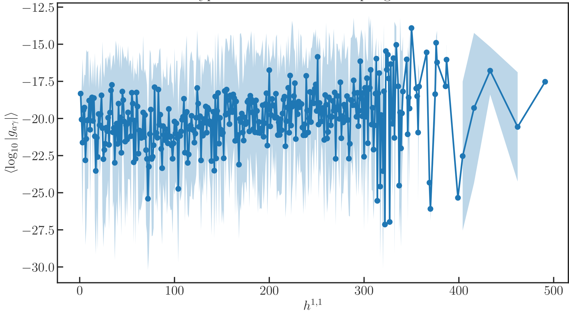
Typical Axion-Photon Coupling vs h^{1,1}
