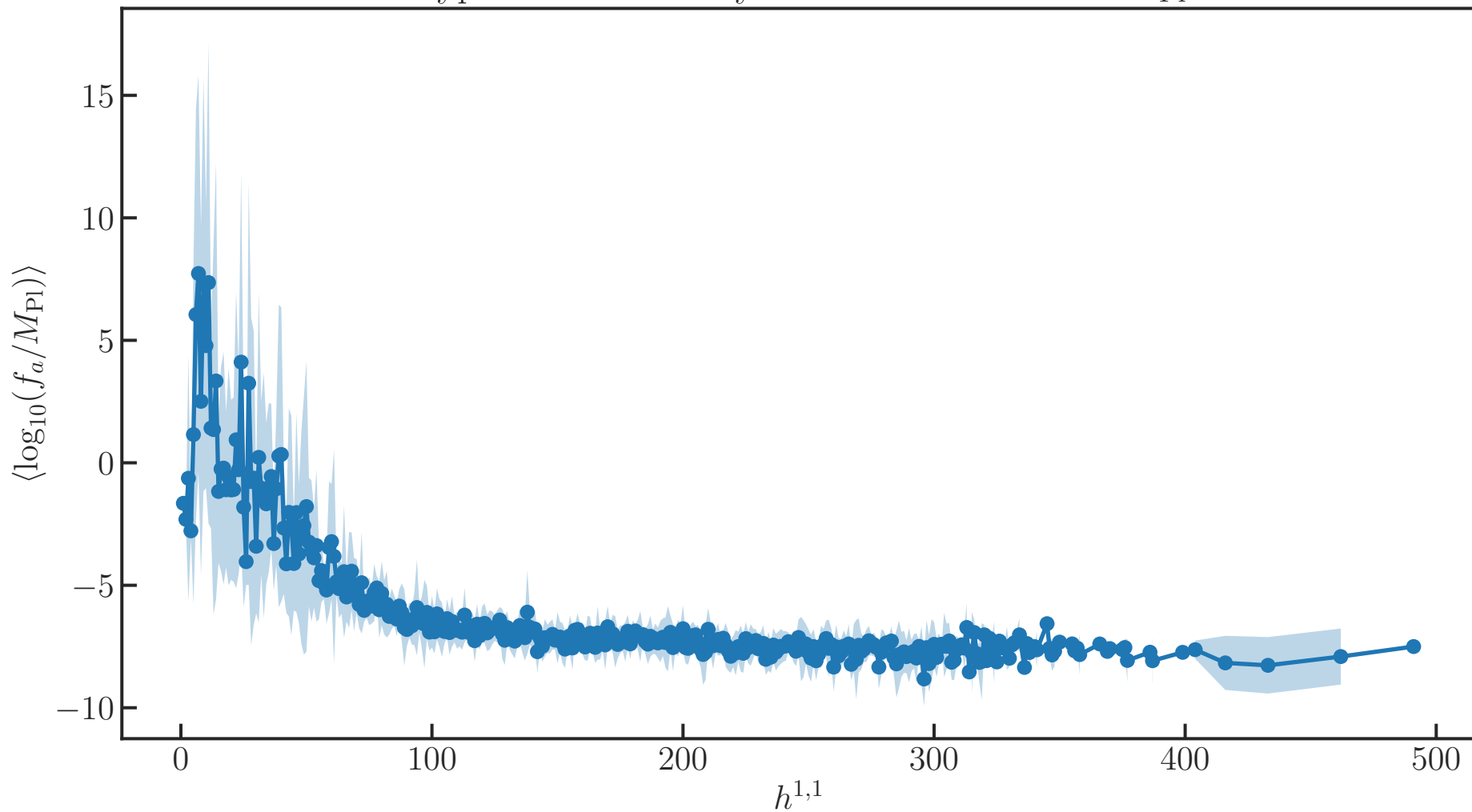
Typical Axion Decay Constant Relative to M_{\text{Pl}}
