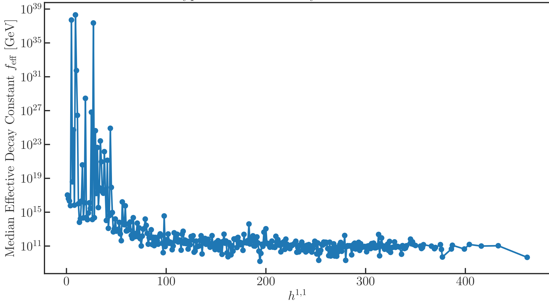
Typical Effective Decay Constant vs h^{1,1}
