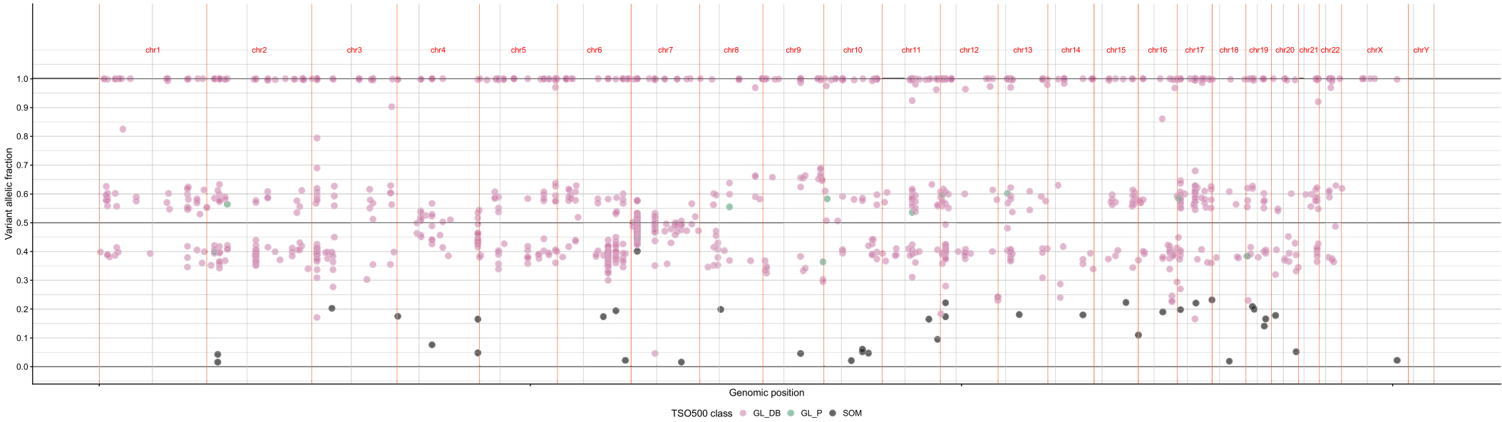
[C1] Allelic fractions of assumed somatic and germline variants in tumor sample IPD2225-D01-P01-A08 (variants at genomic sites with read depth < 50 have been excluded)
