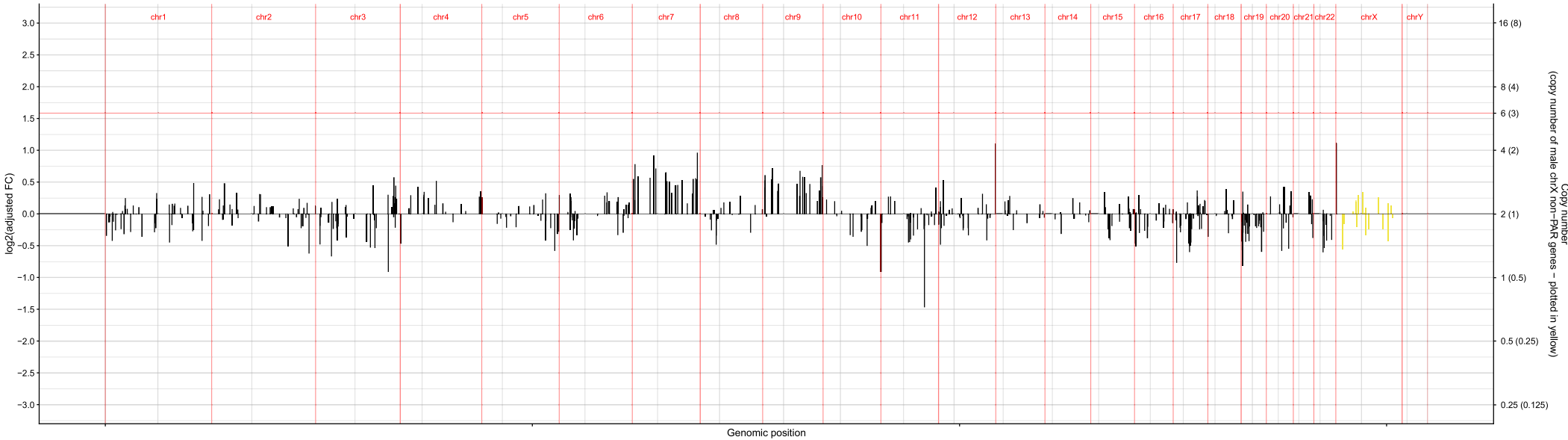
[B3] Copy number status along the genome – bin-wise values for tumor sample IPD2225-D01-P01-A08; tumor content adjustment applied (assumed tumor cell fraction: 0.5)
