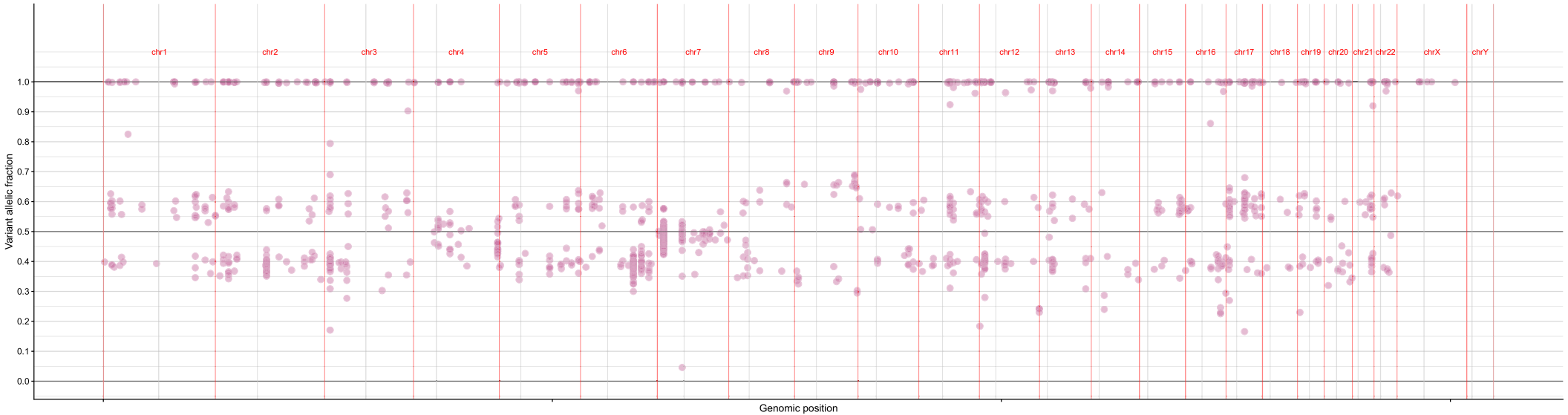
[C4] Allelic fractions of assumed germline (GL_DB) variants in tumor sample IPD2225-D01-P01-A08 (variants at genomic sites with read depth < 50 have been excluded)
