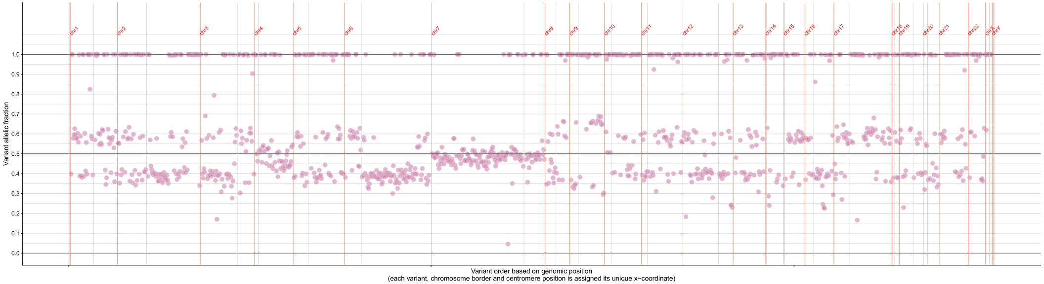
[C3] Allelic fractions of assumed germline (GL_DB) variants in tumor sample IPD2225-D01-P01-A08 (variants at genomic sites with read depth < 50 have been excluded)
