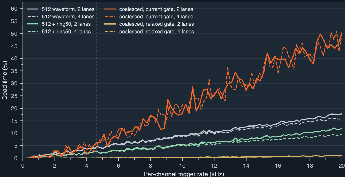
Transport scaling: 2 lanes (20 ch/lane) versus 4 lanes (10 ch/lane)
